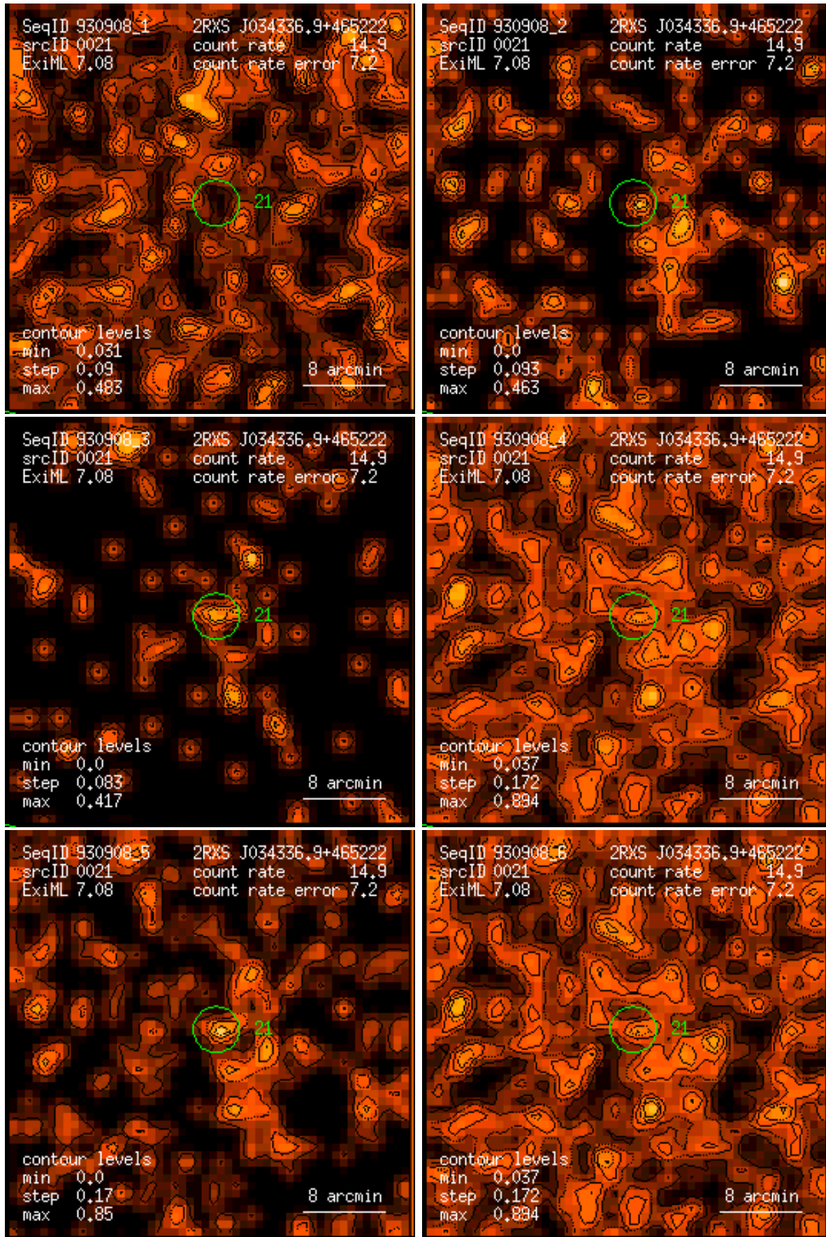
Figure 21: RASS 930908: detection 0021: band rate images, Gaussian filter: (1) PSPC channels 11 – 41, (2) 52 – 90, (3) 91 – 201, (4) 11 – 235, (5) 52 – 201, (6) 11 – 201. Broad band rates in counts/ks. Band rate contour levels in counts/ks/arcmin 2 .
