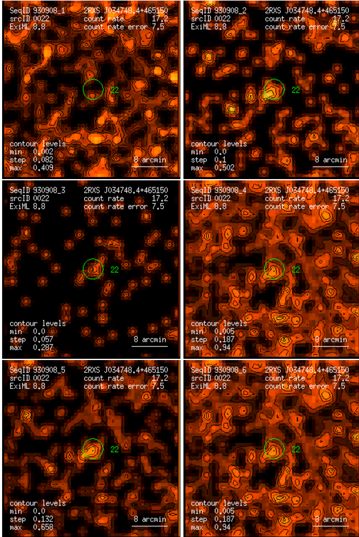
Figure 22: RASS 930908: detection 0022: band rate images, Gaussian filter: (1) PSPC channels 11 – 41, (2) 52 – 90, (3) 91 – 201, (4) 11 – 235, (5) 52 – 201, (6) 11 – 201. Broad band rates in counts/ks. Band rate contour levels in counts/ks/arcmin 2 .
