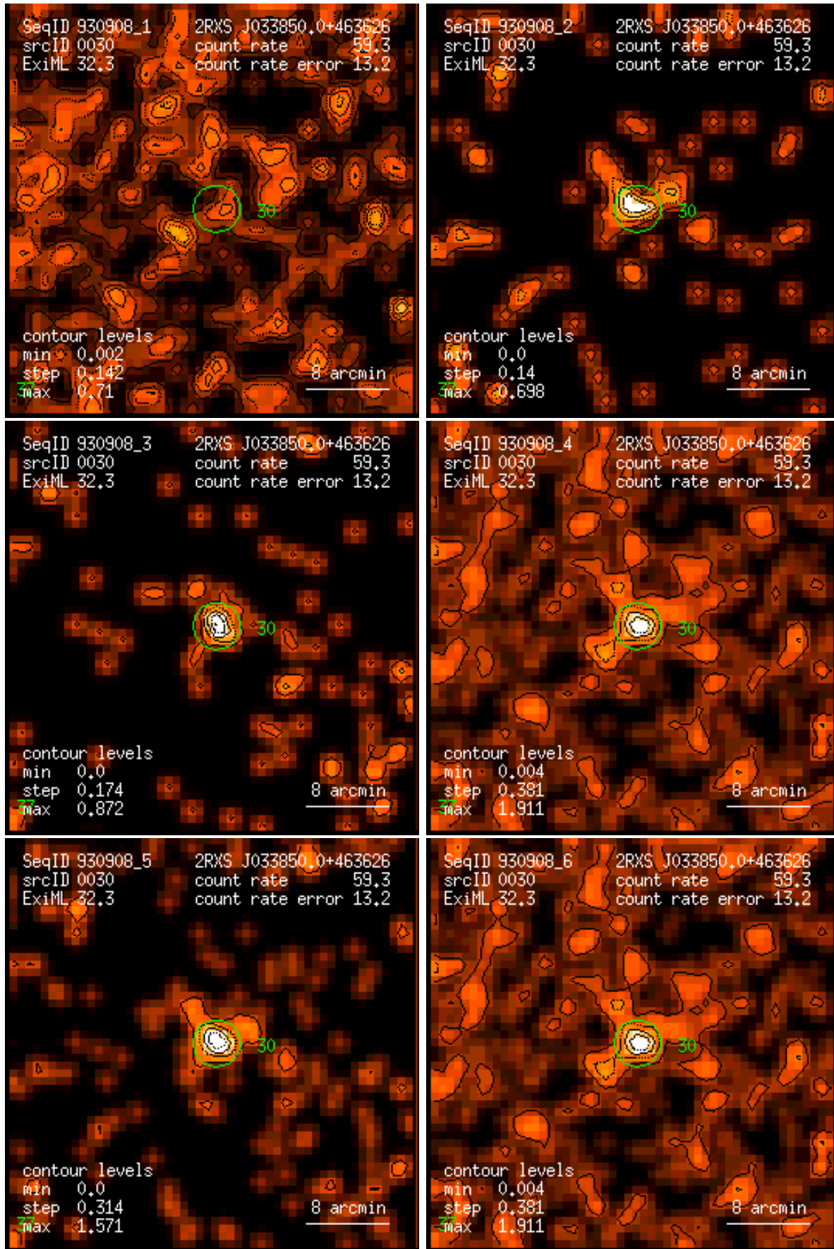
Figure 30: RASS 930908: detection 0030: band rate images, Gaussian filter: (1) PSPC channels 11 – 41, (2) 52 – 90, (3) 91 – 201, (4) 11 – 235, (5) 52 – 201, (6) 11 – 201. Broad band rates in counts/ks. Band rate contour levels in counts/ks/arcmin 2 .
