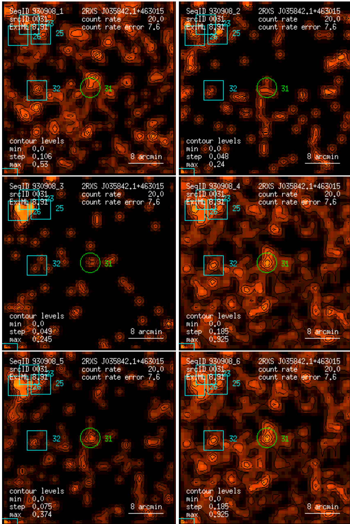
Figure 31: RASS 930908: detection 0031: band rate images, Gaussian filter: (1) PSPC channels 11 – 41, (2) 52 – 90, (3) 91 – 201, (4) 11 – 235, (5) 52 – 201, (6) 11 – 201. Broad band rates in counts/ks. Band rate contour levels in counts/ks/arcmin 2 .
