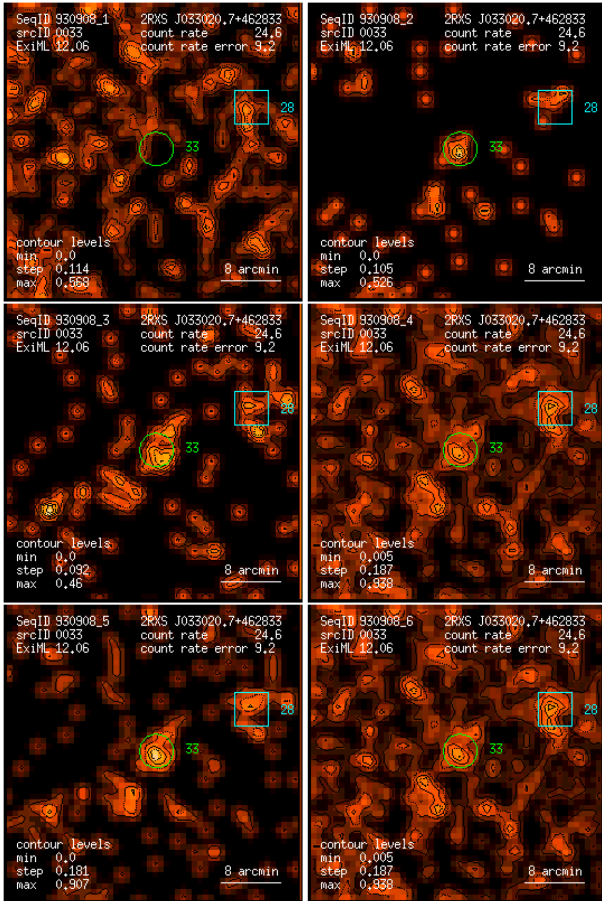
Figure 33: RASS 930908: detection 0033: band rate images, Gaussian filter: (1) PSPC channels 11 – 41, (2) 52 – 90, (3) 91 – 201, (4) 11 – 235, (5) 52 – 201, (6) 11 – 201. Broad band rates in counts/ks. Band rate contour levels in counts/ks/arcmin 2 .
