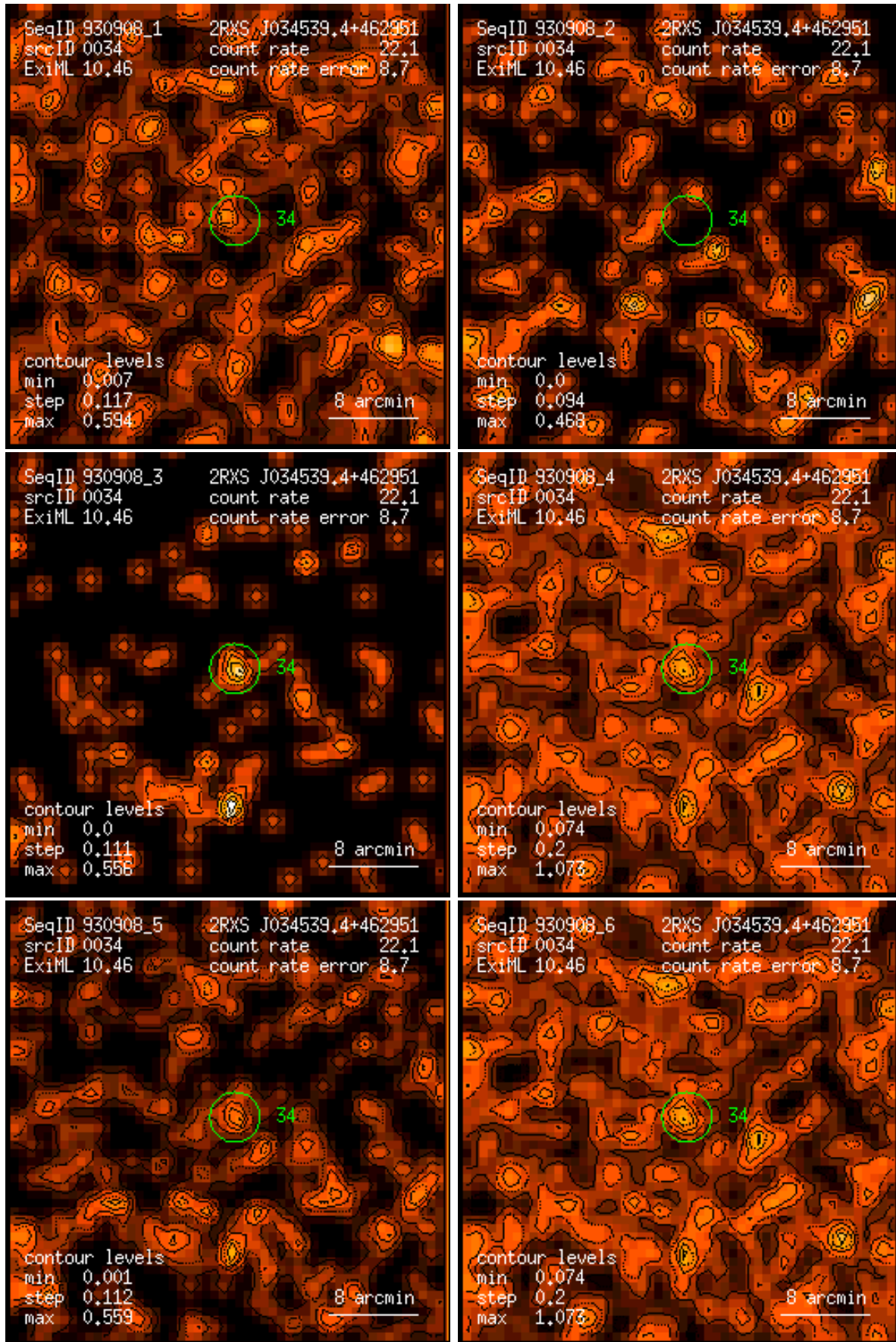
Figure 34: RASS 930908: detection 0034: band rate images, Gaussian filter: (1) PSPC channels 11 – 41, (2) 52 – 90, (3) 91 – 201, (4) 11 – 235, (5) 52 – 201, (6) 11 – 201. Broad band rates in counts/ks. Band rate contour levels in counts/ks/arcmin 2 .
