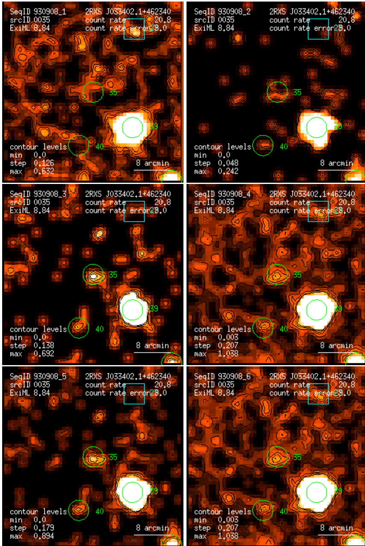
Figure 35: RASS 930908: detection 0035: band rate images, Gaussian filter: (1) PSPC channels 11 – 41, (2) 52 – 90, (3) 91 – 201, (4) 11 – 235, (5) 52 – 201, (6) 11 – 201. Broad band rates in counts/ks. Band rate contour levels in counts/ks/arcmin 2 .
