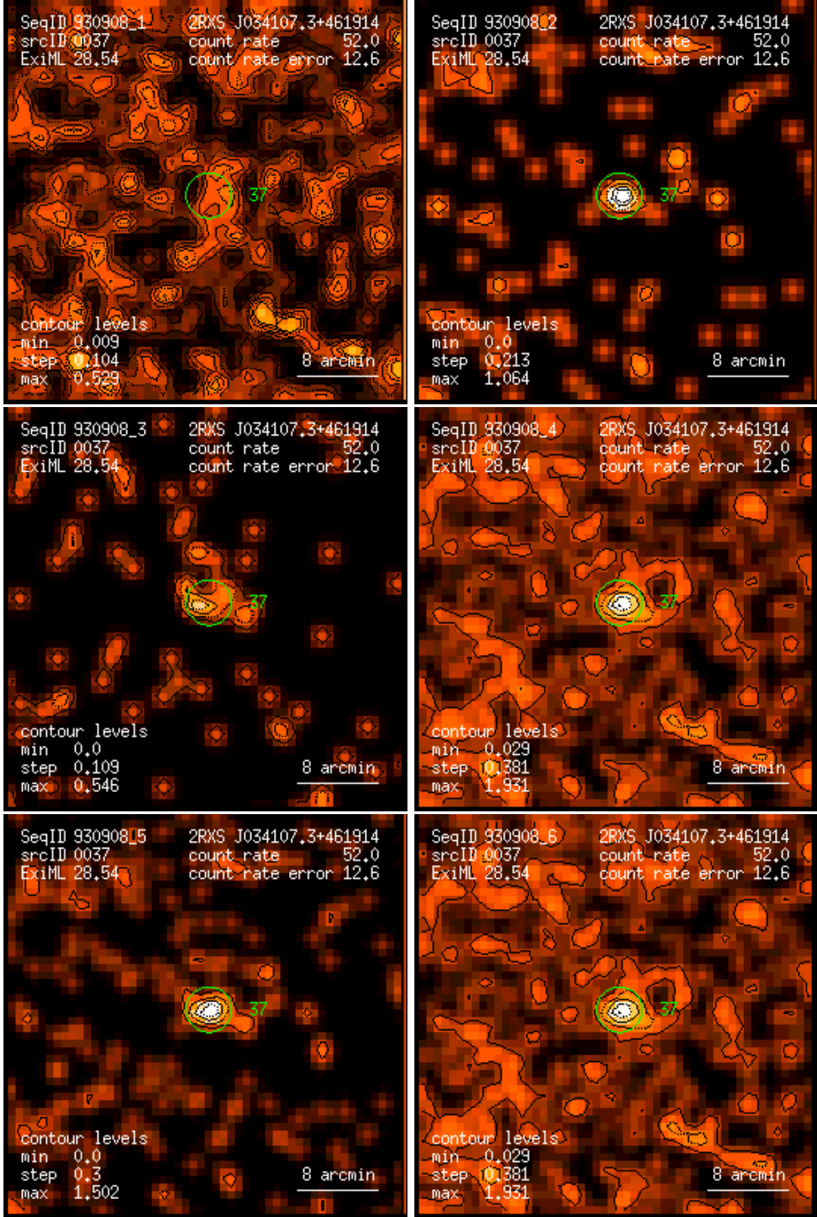
Figure 37: RASS 930908: detection 0037: band rate images, Gaussian filter: (1) PSPC channels 11 – 41, (2) 52 – 90, (3) 91 – 201, (4) 11 – 235, (5) 52 – 201, (6) 11 – 201. Broad band rates in counts/ks. Band rate contour levels in counts/ks/arcmin 2 .
