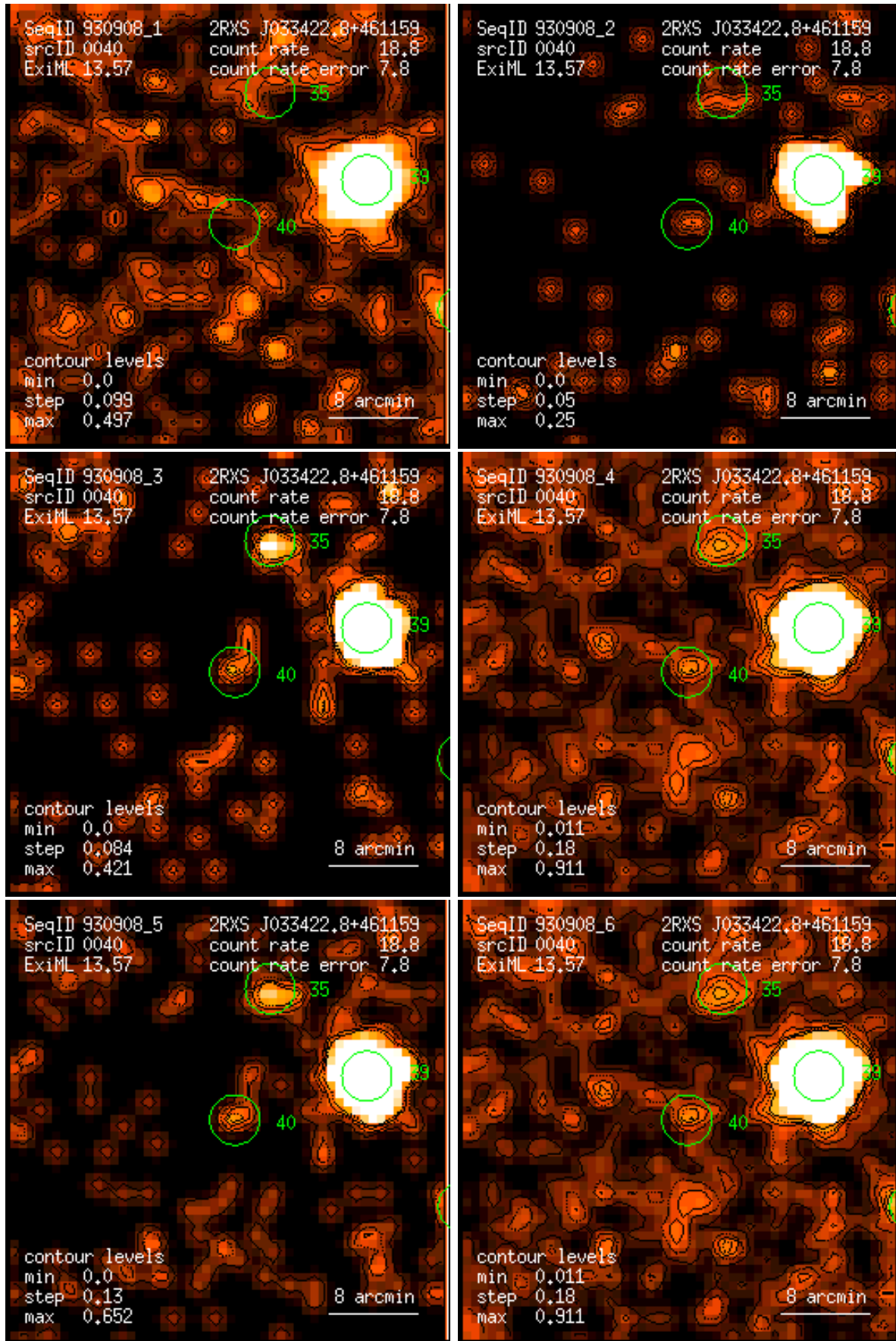
Figure 40: RASS 930908: detection 0040: band rate images, Gaussian filter: (1) PSPC channels 11 – 41, (2) 52 – 90, (3) 91 – 201, (4) 11 – 235, (5) 52 – 201, (6) 11 – 201. Broad band rates in counts/ks. Band rate contour levels in counts/ks/arcmin 2 .
