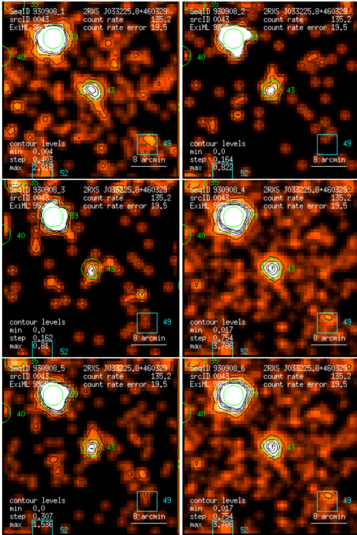
Figure 43: RASS 930908: detection 0043: band rate images, Gaussian filter: (1) PSPC channels 11 – 41, (2) 52 – 90, (3) 91 – 201, (4) 11 – 235, (5) 52 – 201, (6) 11 – 201. Broad band rates in counts/ks. Band rate contour levels in counts/ks/arcmin 2 .
