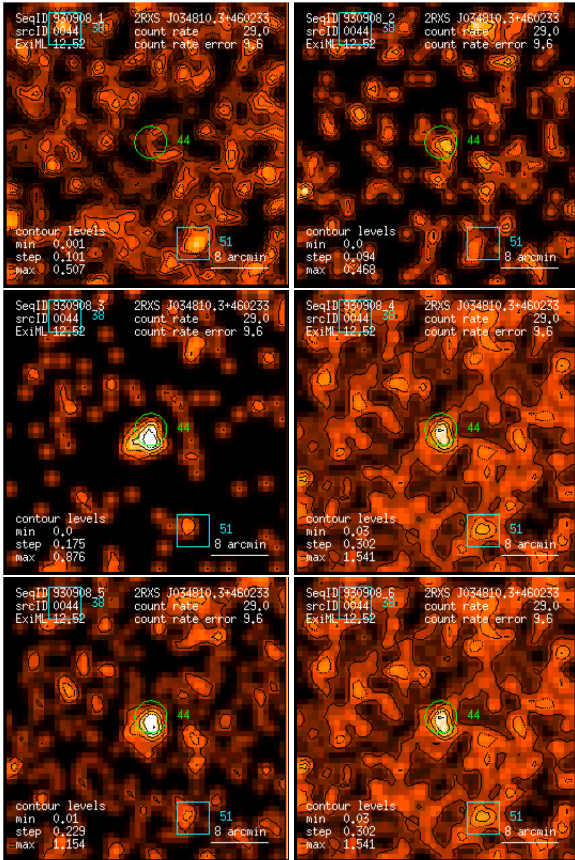
Figure 44: RASS 930908: detection 0044: band rate images, Gaussian filter: (1) PSPC channels 11 – 41, (2) 52 – 90, (3) 91 – 201, (4) 11 – 235, (5) 52 – 201, (6) 11 – 201. Broad band rates in counts/ks. Band rate contour levels in counts/ks/arcmin 2 .
