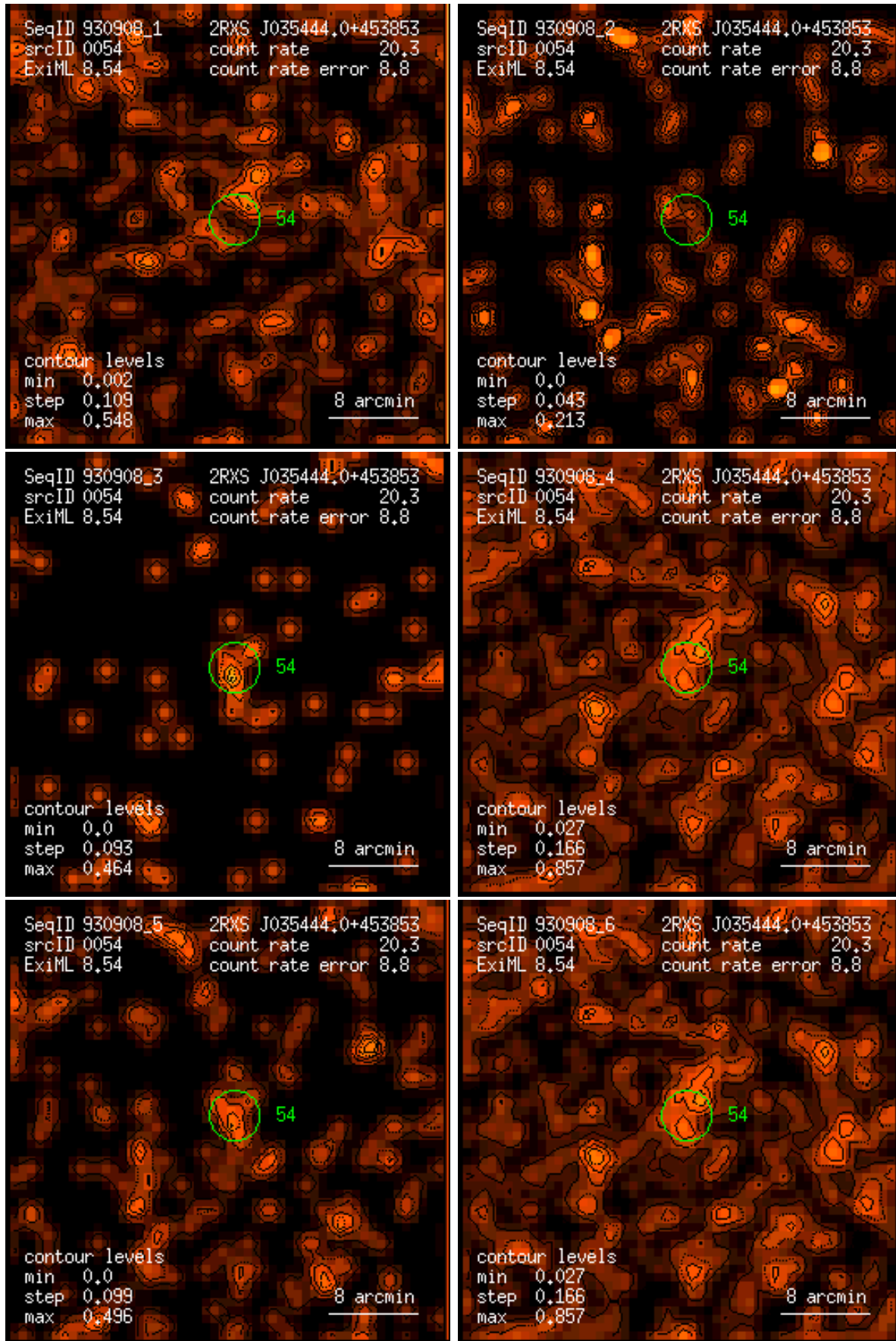
Figure 54: RASS 930908: detection 0054: band rate images, Gaussian filter: (1) PSPC channels 11 – 41, (2) 52 – 90, (3) 91 – 201, (4) 11 – 235, (5) 52 – 201, (6) 11 – 201. Broad band rates in counts/ks. Band rate contour levels in counts/ks/arcmin 2 .
