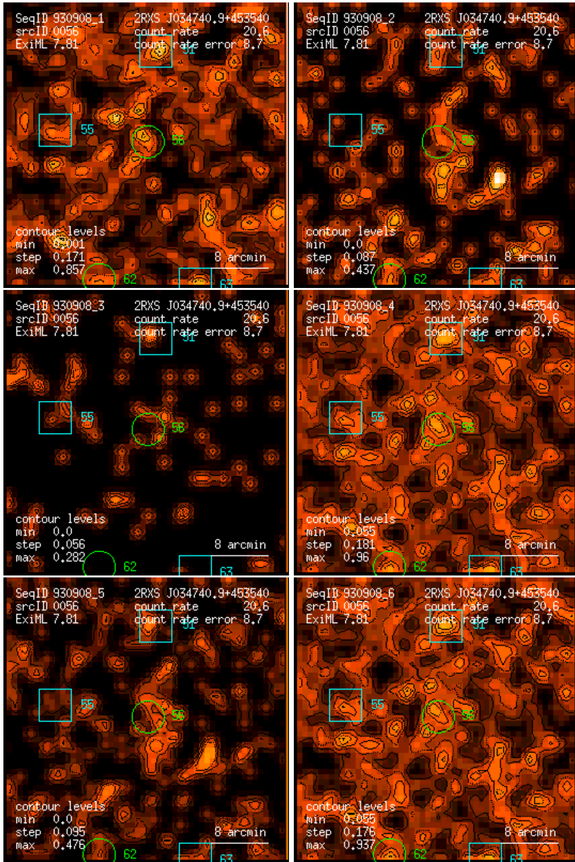
Figure 56: RASS 930908: detection 0056: band rate images, Gaussian filter: (1) PSPC channels 11 – 41, (2) 52 – 90, (3) 91 – 201, (4) 11 – 235, (5) 52 – 201, (6) 11 – 201. Broad band rates in counts/ks. Band rate contour levels in counts/ks/arcmin 2 .
