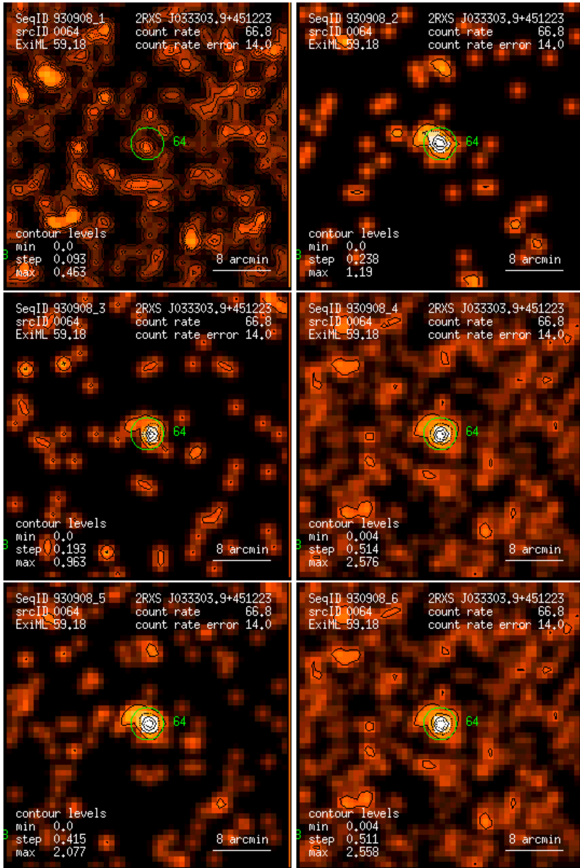
Figure 64: RASS 930908: detection 0064: band rate images, Gaussian filter: (1) PSPC channels 11 – 41, (2) 52 – 90, (3) 91 – 201, (4) 11 – 235, (5) 52 – 201, (6) 11 – 201. Broad band rates in counts/ks. Band rate contour levels in counts/ks/arcmin 2 .
