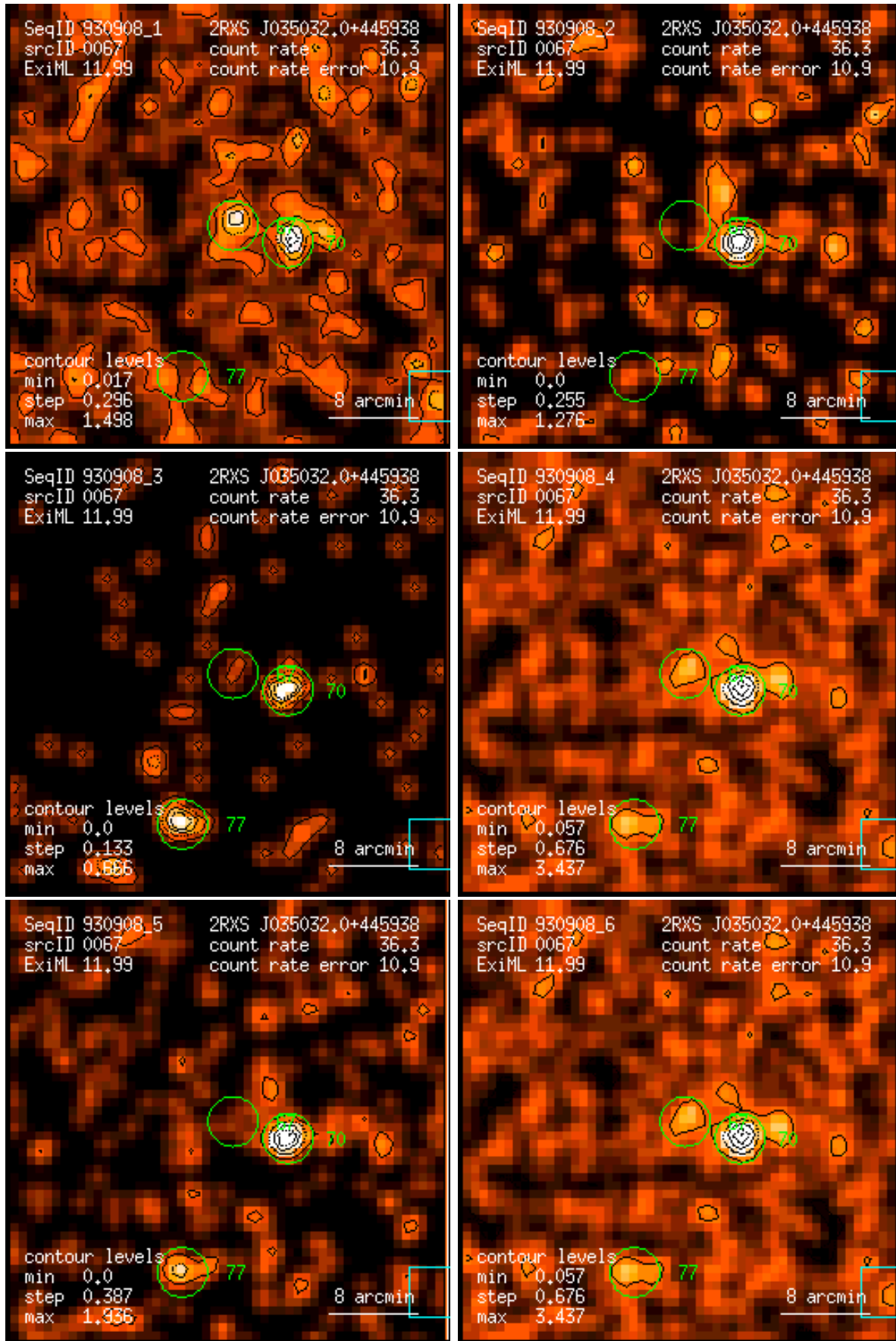
Figure 67: RASS 930908: detection 0067: band rate images, Gaussian filter: (1) PSPC channels 11 – 41, (2) 52 – 90, (3) 91 – 201, (4) 11 – 235, (5) 52 – 201, (6) 11 – 201. Broad band rates in counts/ks. Band rate contour levels in counts/ks/arcmin 2 .
