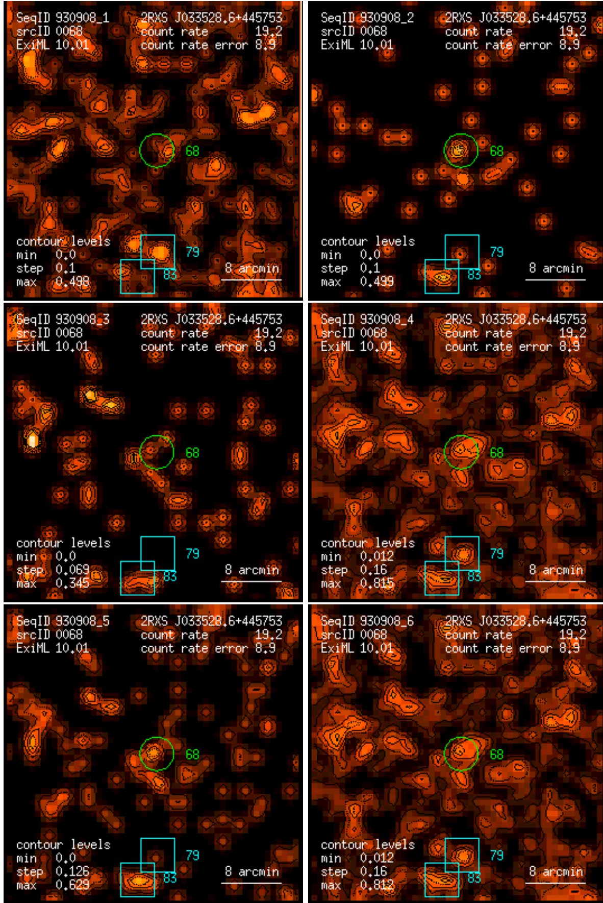
Figure 68: RASS 930908: detection 0068: band rate images, Gaussian filter: (1) PSPC channels 11 – 41, (2) 52 – 90, (3) 91 – 201, (4) 11 – 235, (5) 52 – 201, (6) 11 – 201. Broad band rates in counts/ks. Band rate contour levels in counts/ks/arcmin 2 .
