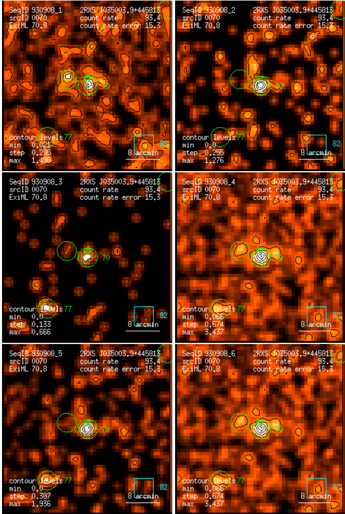
Figure 70: RASS 930908: detection 0070: band rate images, Gaussian filter: (1) PSPC channels 11 – 41, (2) 52 – 90, (3) 91 – 201, (4) 11 – 235, (5) 52 – 201, (6) 11 – 201. Broad band rates in counts/ks. Band rate contour levels in counts/ks/arcmin 2 .
