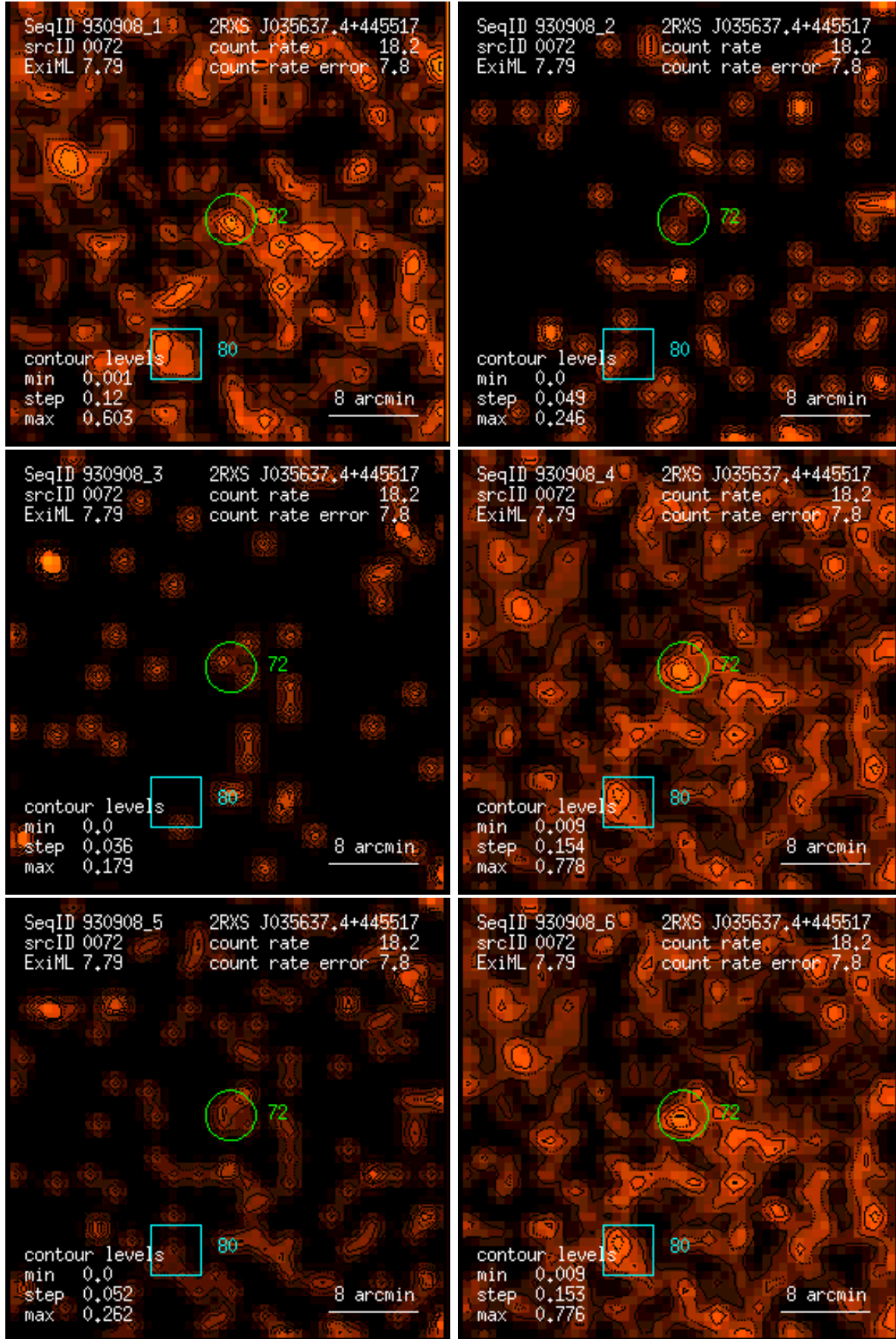
Figure 72: RASS 930908: detection 0072: band rate images, Gaussian filter: (1) PSPC channels 11 – 41, (2) 52 – 90, (3) 91 – 201, (4) 11 – 235, (5) 52 – 201, (6) 11 – 201. Broad band rates in counts/ks. Band rate contour levels in counts/ks/arcmin 2 .
