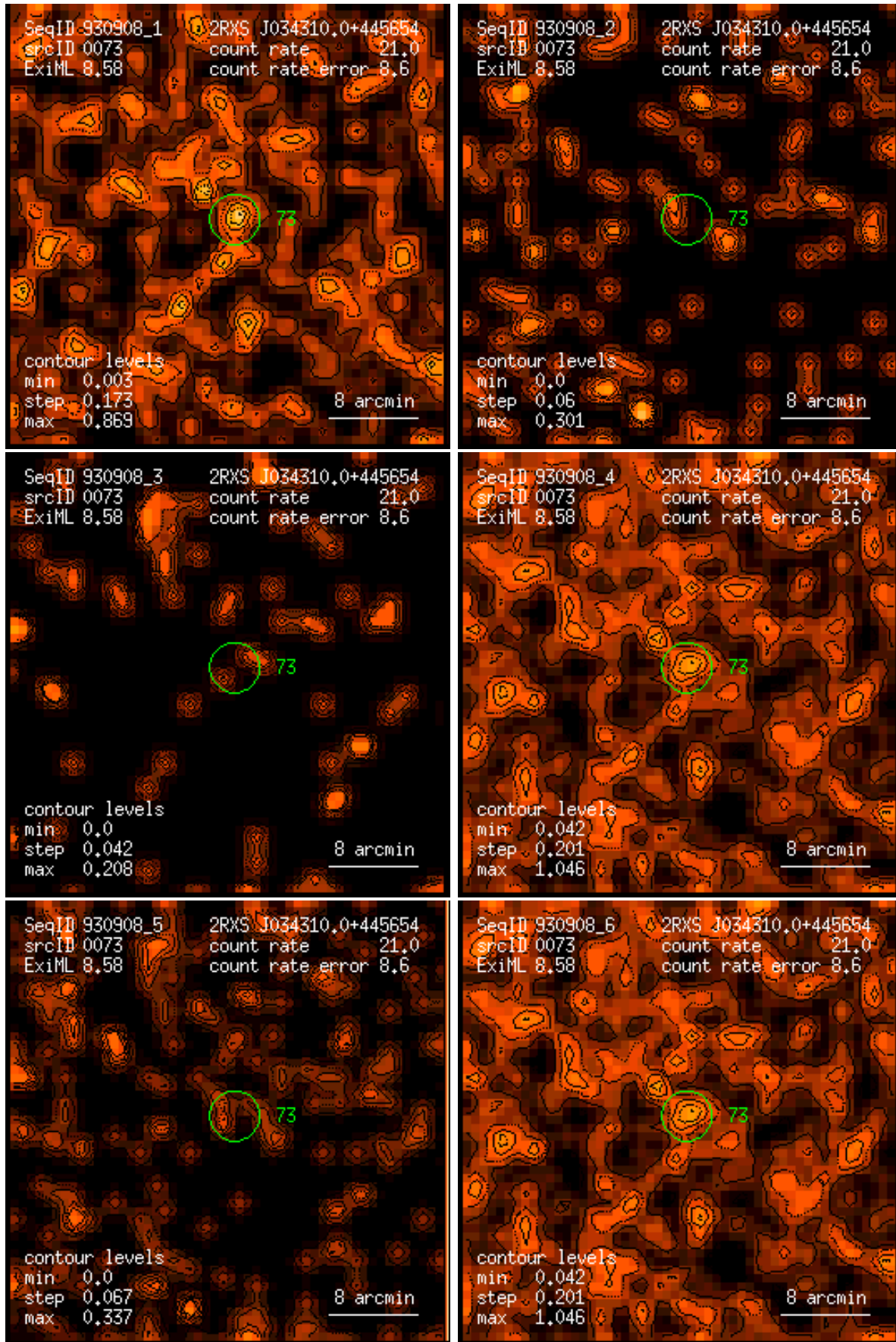
Figure 73: RASS 930908: detection 0073: band rate images, Gaussian filter: (1) PSPC channels 11 – 41, (2) 52 – 90, (3) 91 – 201, (4) 11 – 235, (5) 52 – 201, (6) 11 – 201. Broad band rates in counts/ks. Band rate contour levels in counts/ks/arcmin 2 .
