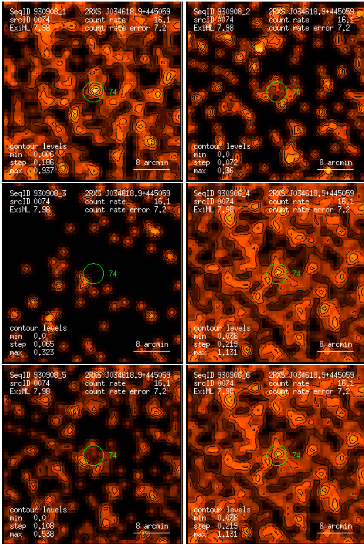
Figure 74: RASS 930908: detection 0074: band rate images, Gaussian filter: (1) PSPC channels 11 – 41, (2) 52 – 90, (3) 91 – 201, (4) 11 – 235, (5) 52 – 201, (6) 11 – 201. Broad band rates in counts/ks. Band rate contour levels in counts/ks/arcmin 2 .
