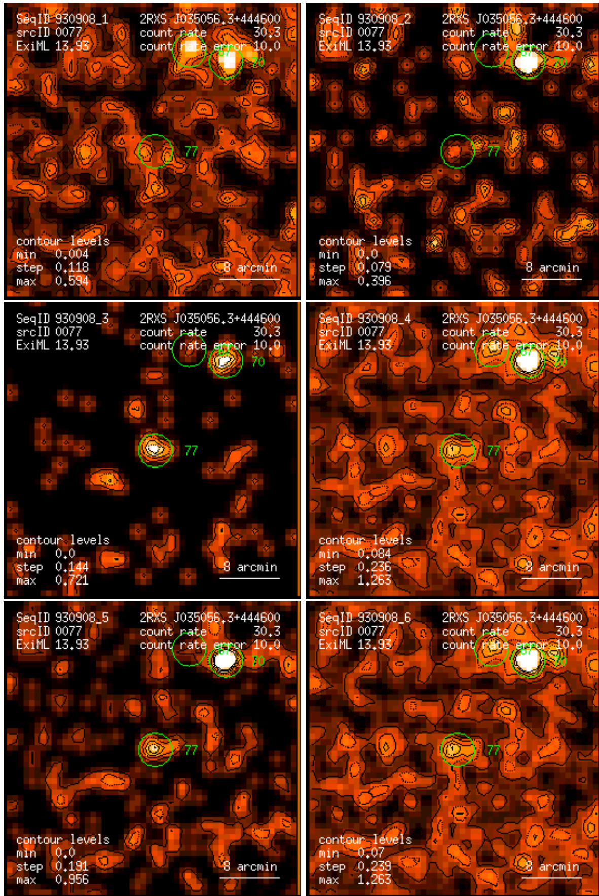
Figure 77: RASS 930908: detection 0077: band rate images, Gaussian filter: (1) PSPC channels 11 – 41, (2) 52 – 90, (3) 91 – 201, (4) 11 – 235, (5) 52 – 201, (6) 11 – 201. Broad band rates in counts/ks. Band rate contour levels in counts/ks/arcmin 2 .
