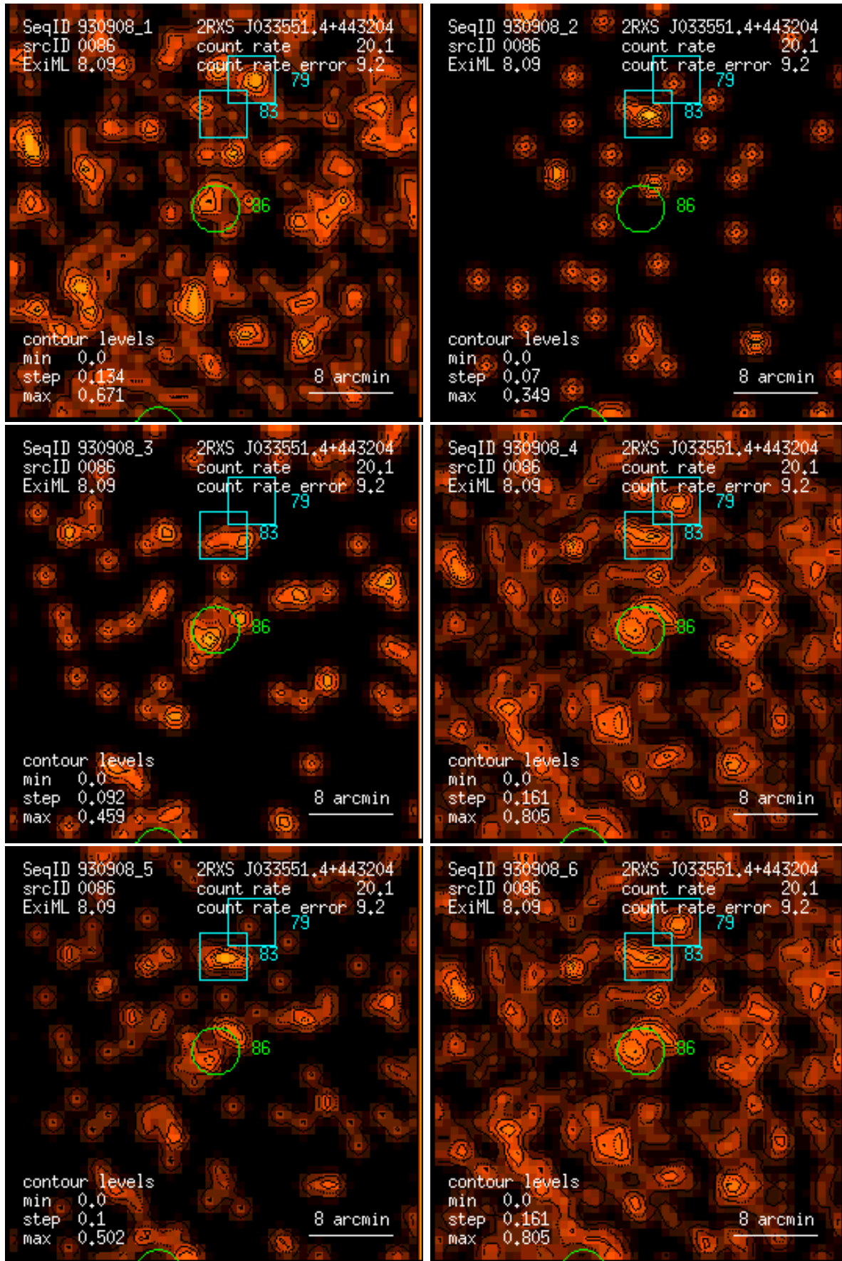
Figure 86: RASS 930908: detection 0086: band rate images, Gaussian filter: (1) PSPC channels 11 – 41, (2) 52 – 90, (3) 91 – 201, (4) 11 – 235, (5) 52 – 201, (6) 11 – 201. Broad band rates in counts/ks. Band rate contour levels in counts/ks/arcmin 2 .
