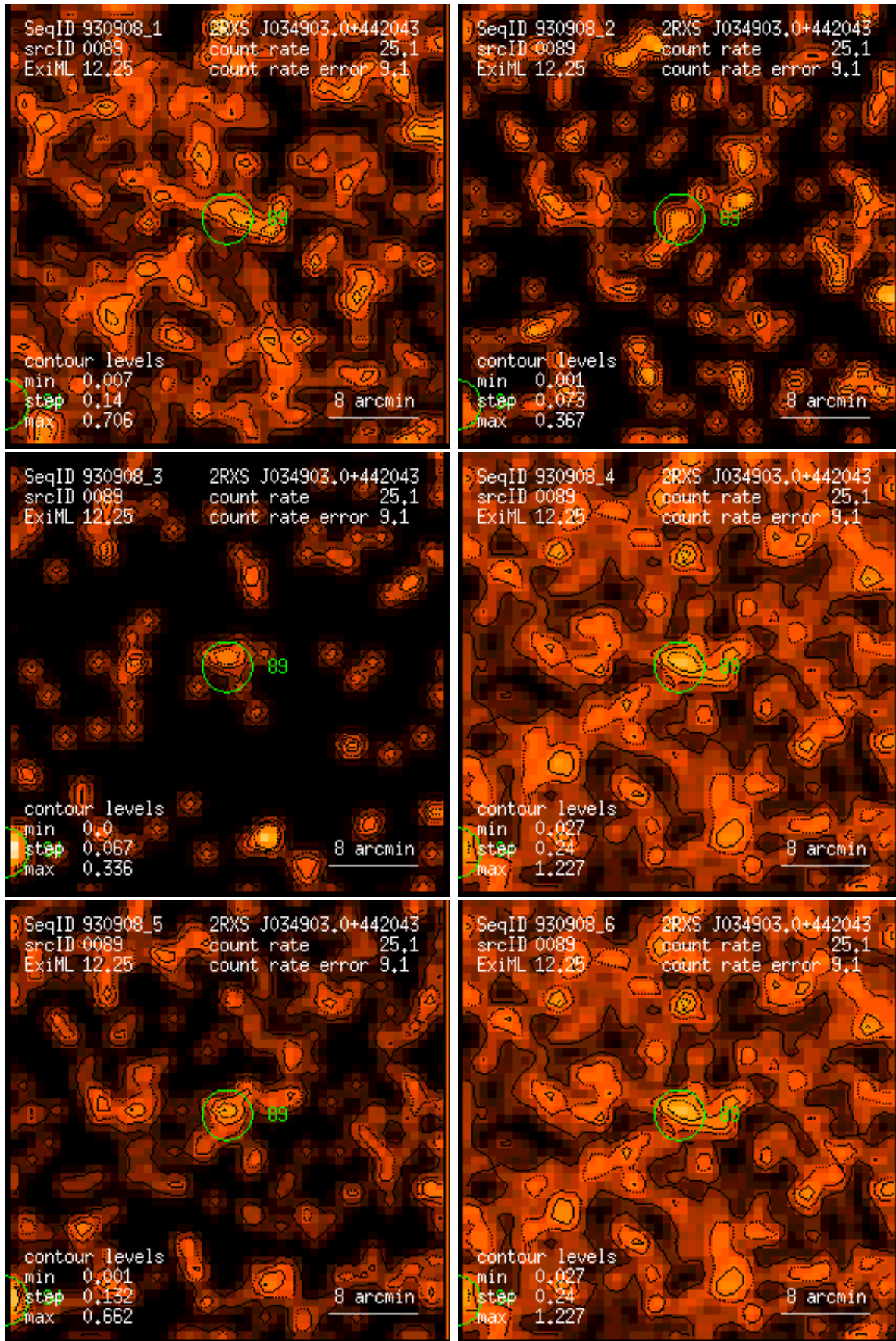
Figure 89: RASS 930908: detection 0089: band rate images, Gaussian filter: (1) PSPC channels 11 – 41, (2) 52 – 90, (3) 91 – 201, (4) 11 – 235, (5) 52 – 201, (6) 11 – 201. Broad band rates in counts/ks. Band rate contour levels in counts/ks/arcmin 2 .
