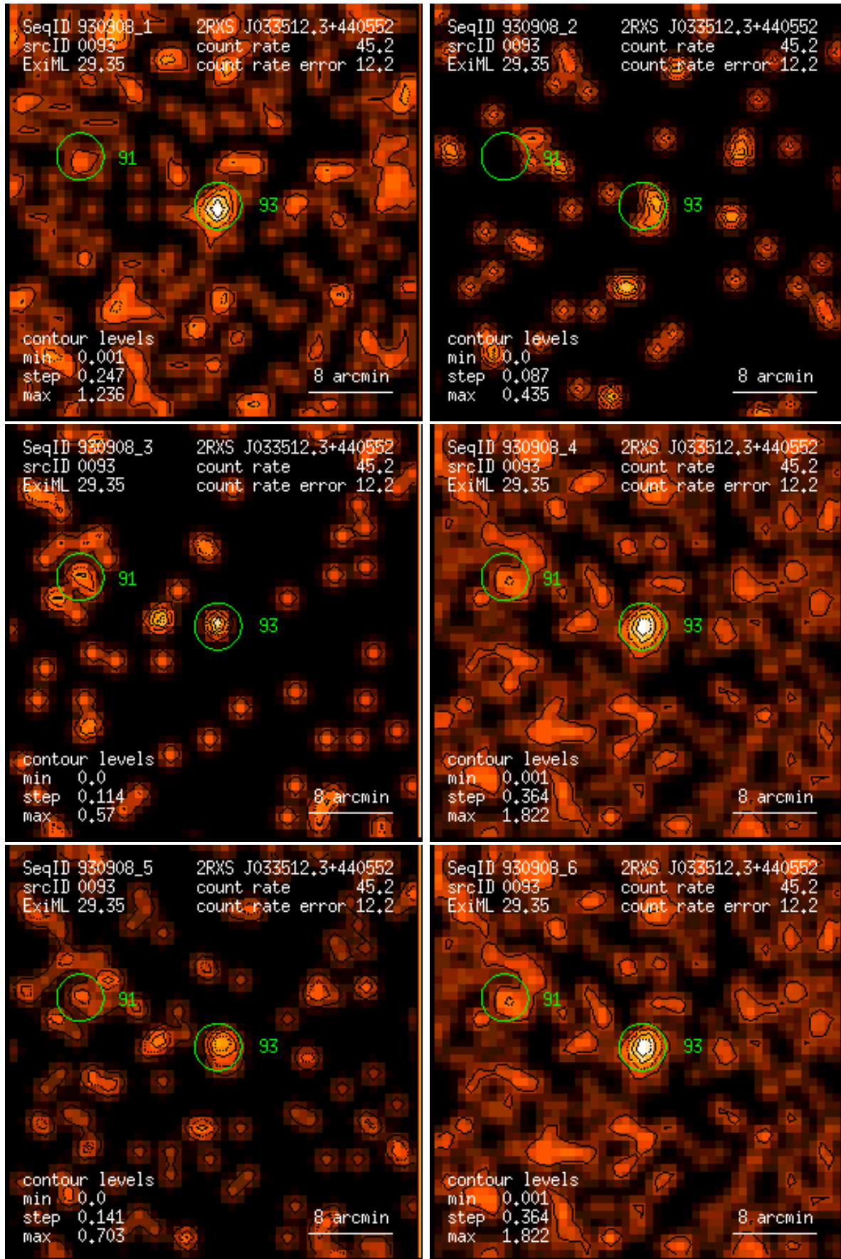
Figure 93: RASS 930908: detection 0093: band rate images, Gaussian filter: (1) PSPC channels 11 – 41, (2) 52 – 90, (3) 91 – 201, (4) 11 – 235, (5) 52 – 201, (6) 11 – 201. Broad band rates in counts/ks. Band rate contour levels in counts/ks/arcmin 2 .
