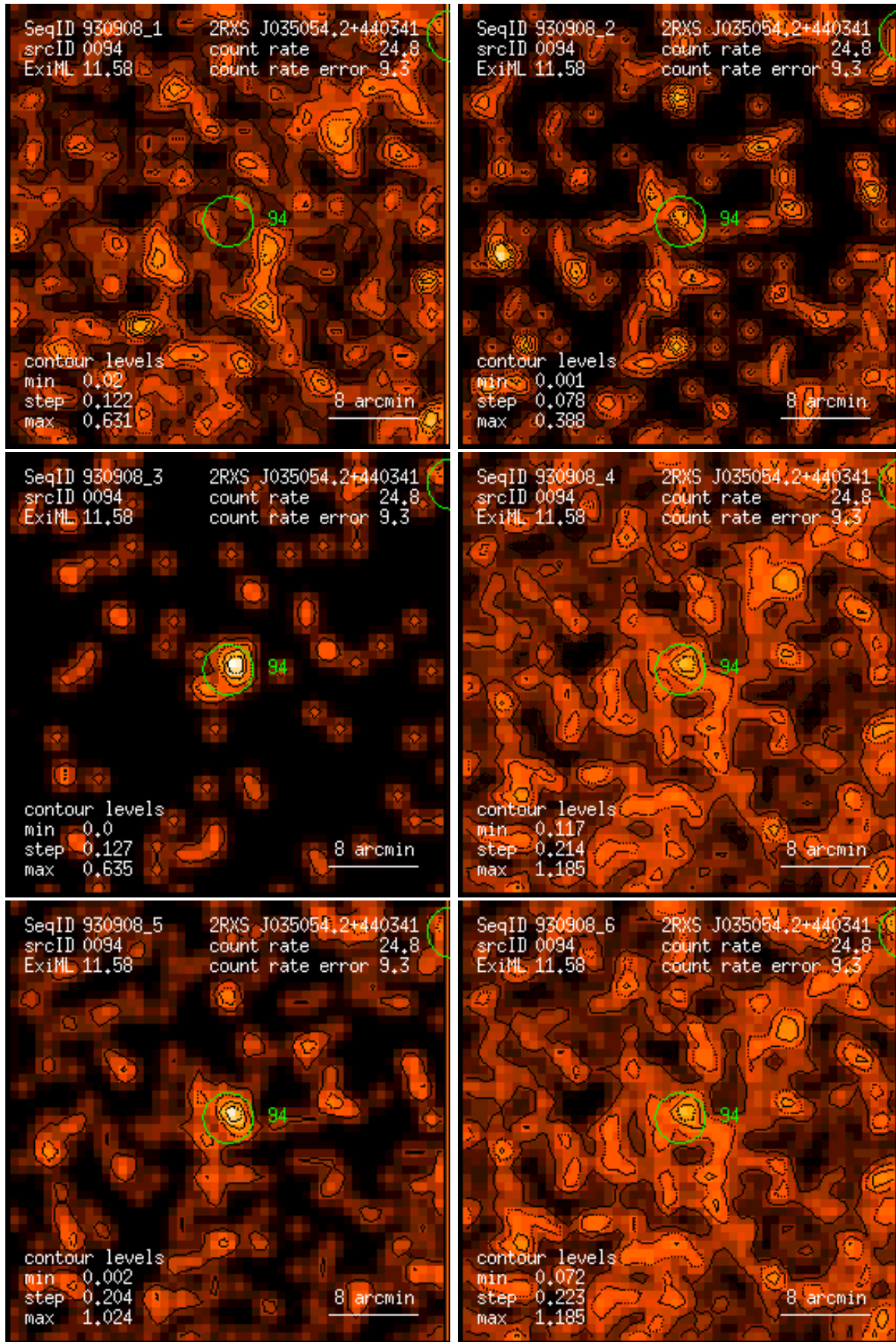
Figure 94: RASS 930908: detection 0094: band rate images, Gaussian filter: (1) PSPC channels 11 – 41, (2) 52 – 90, (3) 91 – 201, (4) 11 – 235, (5) 52 – 201, (6) 11 – 201. Broad band rates in counts/ks. Band rate contour levels in counts/ks/arcmin 2 .
