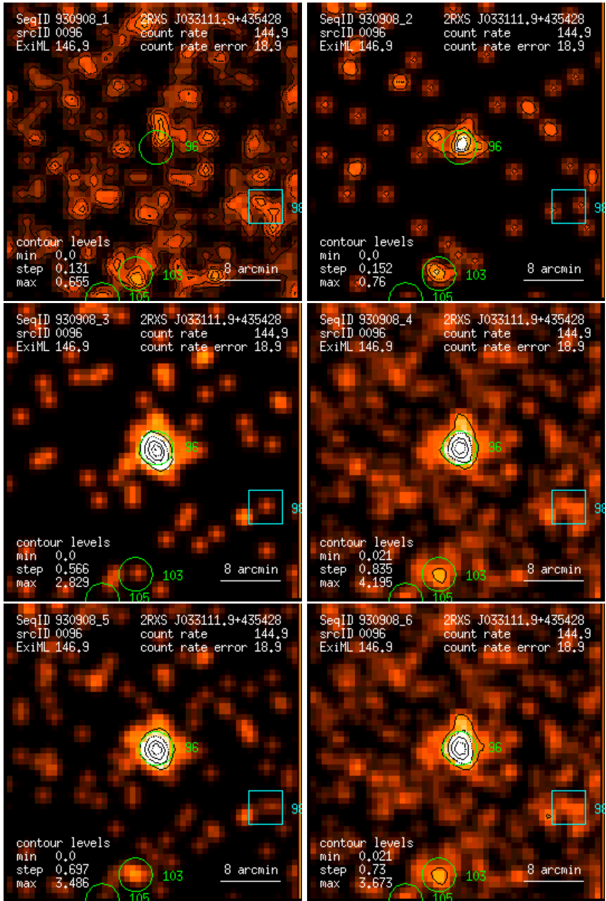
Figure 96: RASS 930908: detection 0096: band rate images, Gaussian filter: (1) PSPC channels 11 – 41, (2) 52 – 90, (3) 91 – 201, (4) 11 – 235, (5) 52 – 201, (6) 11 – 201. Broad band rates in counts/ks. Band rate contour levels in counts/ks/arcmin 2 .
