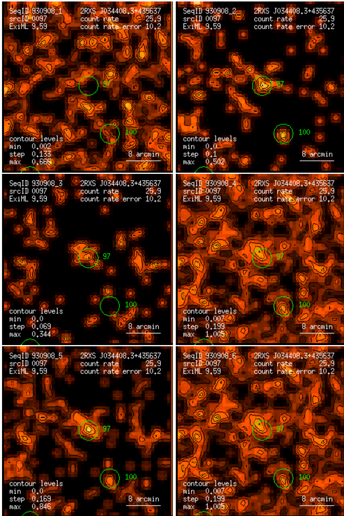
Figure 97: RASS 930908: detection 0097: band rate images, Gaussian filter: (1) PSPC channels 11 – 41, (2) 52 – 90, (3) 91 – 201, (4) 11 – 235, (5) 52 – 201, (6) 11 – 201. Broad band rates in counts/ks. Band rate contour levels in counts/ks/arcmin 2 .
