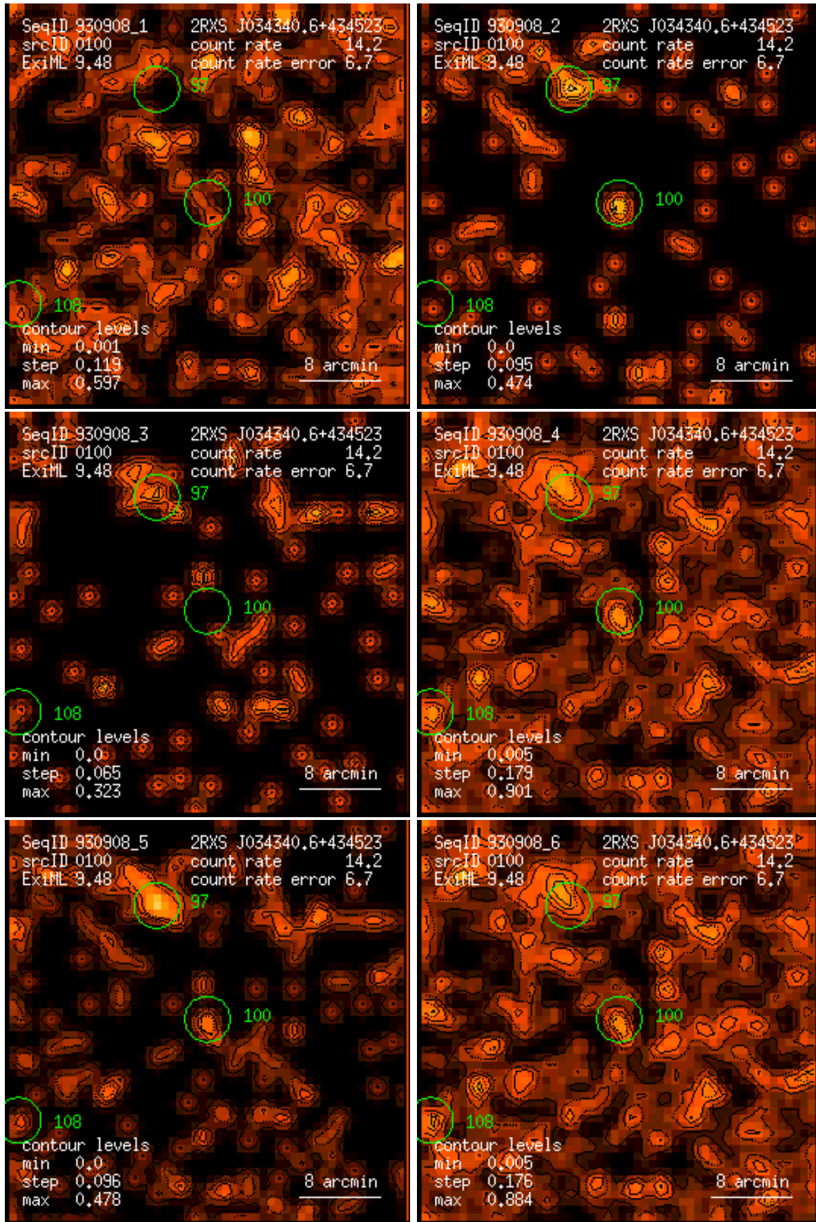
Figure 100: RASS 930908: detection 0100: band rate images, Gaussian filter: (1) PSPC channels 11 – 41, (2) 52 – 90, (3) 91 – 201, (4) 11 – 235, (5) 52 – 201, (6) 11 – 201. Broad band rates in counts/ks. Band rate contour levels in counts/ks/arcmin 2 .
