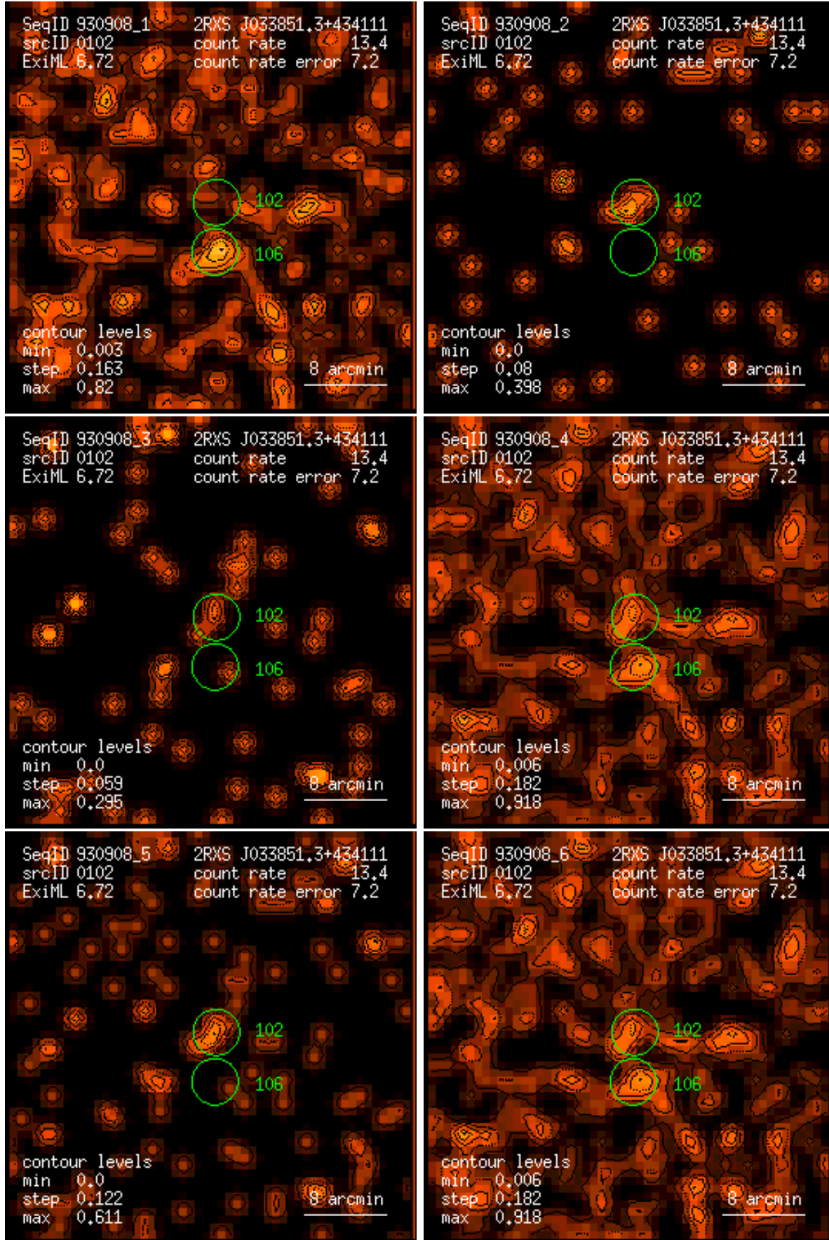
Figure 102: RASS 930908: detection 0102: band rate images, Gaussian filter: (1) PSPC channels 11 – 41, (2) 52 – 90, (3) 91 – 201, (4) 11 – 235, (5) 52 – 201, (6) 11 – 201. Broad band rates in counts/ks. Band rate contour levels in counts/ks/arcmin 2 .
