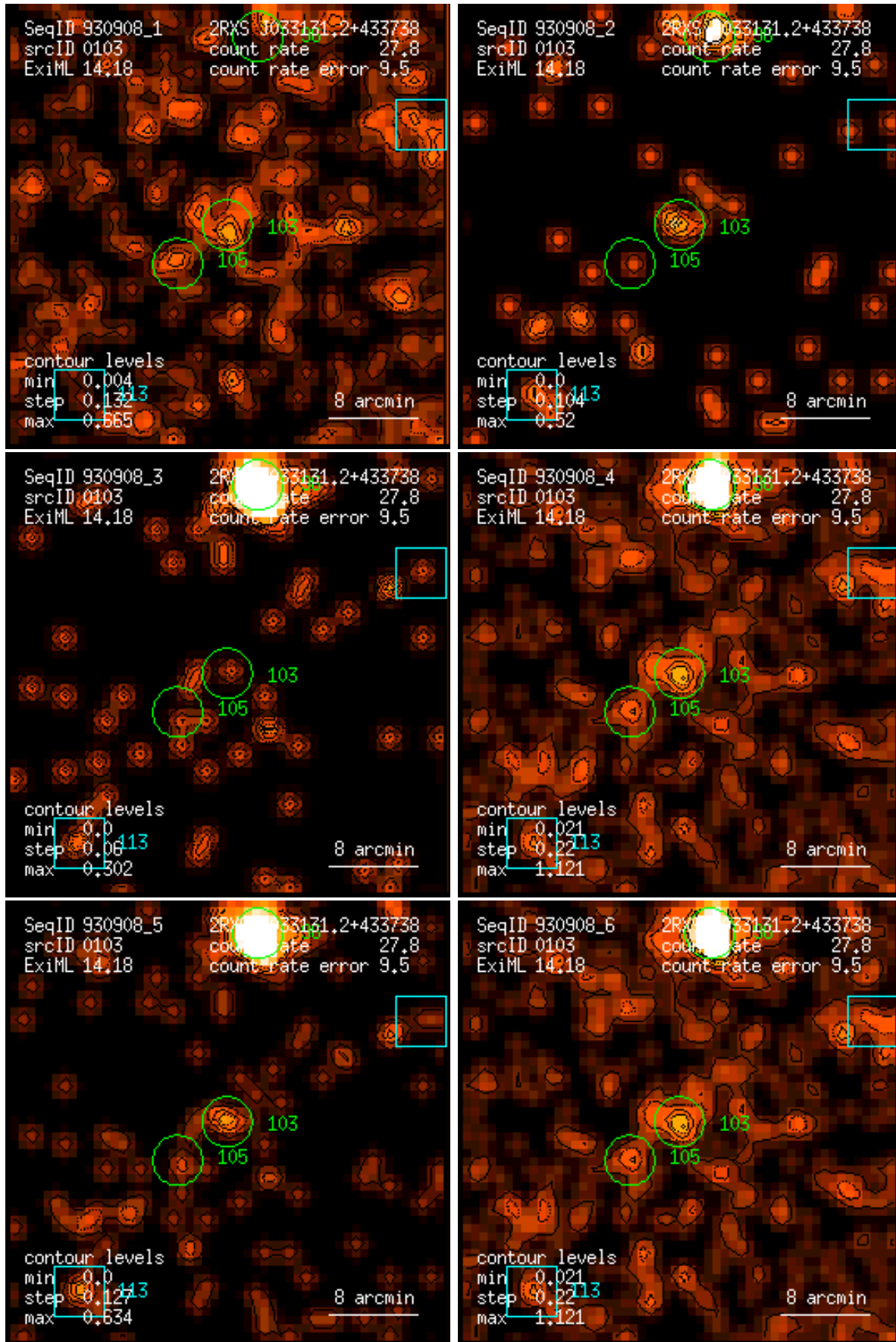
Figure 103: RASS 930908: detection 0103: band rate images, Gaussian filter: (1) PSPC channels 11 – 41, (2) 52 – 90, (3) 91 – 201, (4) 11 – 235, (5) 52 – 201, (6) 11 – 201. Broad band rates in counts/ks. Band rate contour levels in counts/ks/arcmin 2 .
