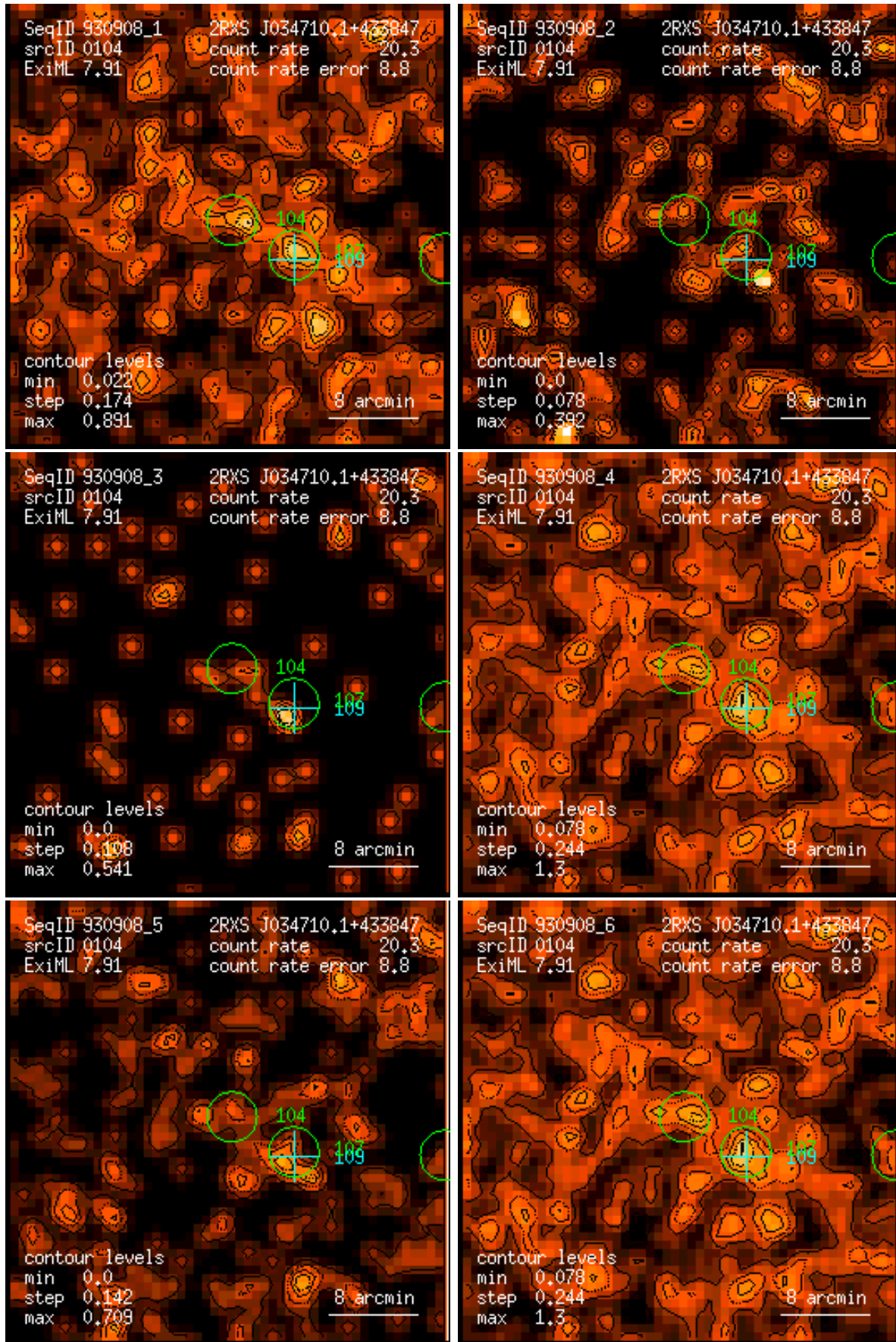
Figure 104: RASS 930908: detection 0104: band rate images, Gaussian filter: (1) PSPC channels 11 – 41, (2) 52 – 90, (3) 91 – 201, (4) 11 – 235, (5) 52 – 201, (6) 11 – 201. Broad band rates in counts/ks. Band rate contour levels in counts/ks/arcmin 2 .
