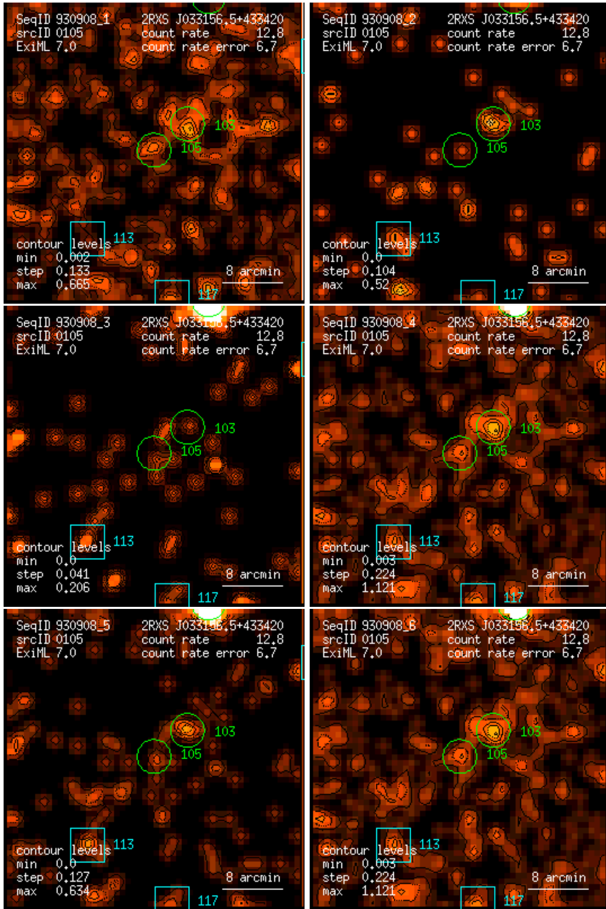
Figure 105: RASS 930908: detection 0105: band rate images, Gaussian filter: (1) PSPC channels 11 – 41, (2) 52 – 90, (3) 91 – 201, (4) 11 – 235, (5) 52 – 201, (6) 11 – 201. Broad band rates in counts/ks. Band rate contour levels in counts/ks/arcmin 2 .
