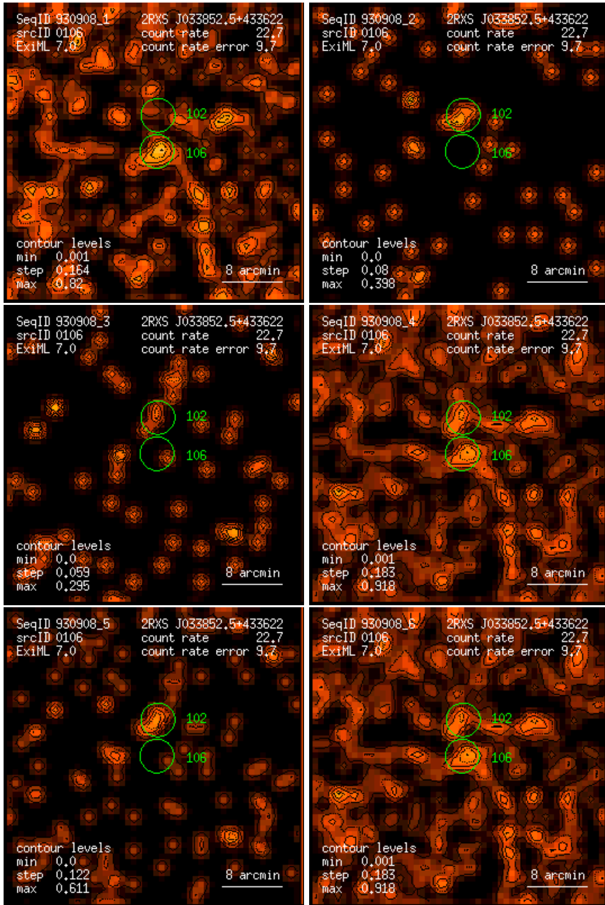
Figure 106: RASS 930908: detection 0106: band rate images, Gaussian filter: (1) PSPC channels 11 – 41, (2) 52 – 90, (3) 91 – 201, (4) 11 – 235, (5) 52 – 201, (6) 11 – 201. Broad band rates in counts/ks. Band rate contour levels in counts/ks/arcmin 2 .
