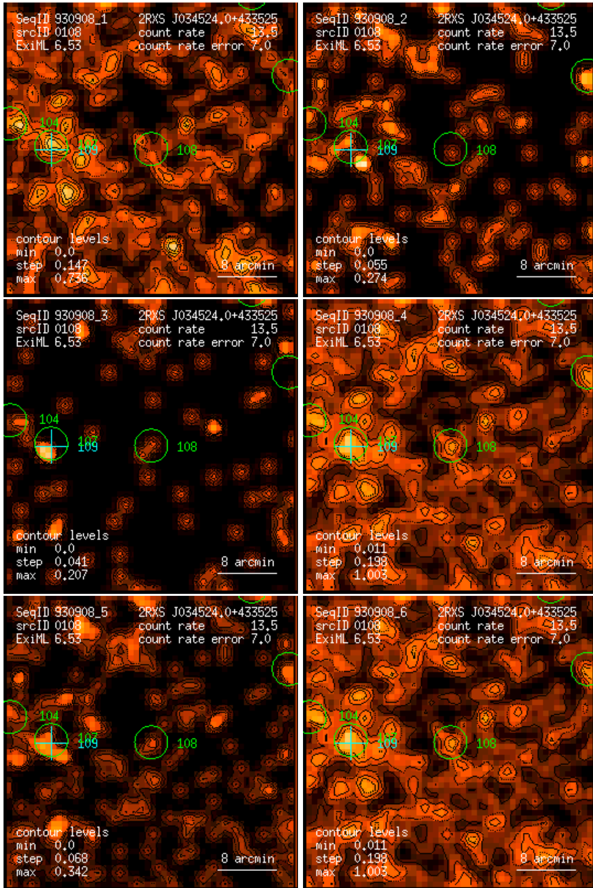
Figure 108: RASS 930908: detection 0108: band rate images, Gaussian filter: (1) PSPC channels 11 – 41, (2) 52 – 90, (3) 91 – 201, (4) 11 – 235, (5) 52 – 201, (6) 11 – 201. Broad band rates in counts/ks. Band rate contour levels in counts/ks/arcmin 2 .
