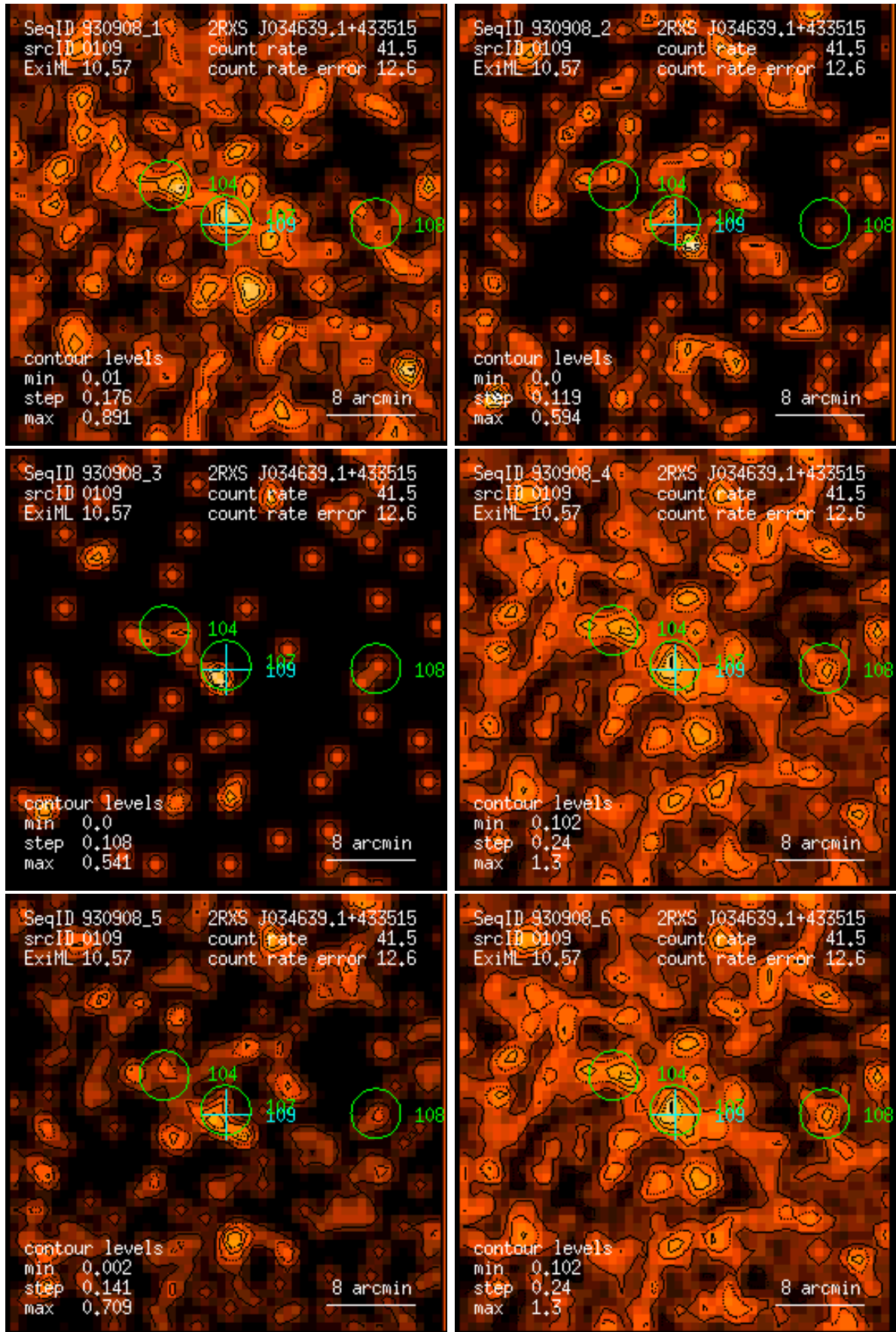
Figure 109: RASS 930908: detection 0109: band rate images, Gaussian filter: (1) PSPC channels 11 – 41, (2) 52 – 90, (3) 91 – 201, (4) 11 – 235, (5) 52 – 201, (6) 11 – 201. Broad band rates in counts/ks. Band rate contour levels in counts/ks/arcmin 2 .
