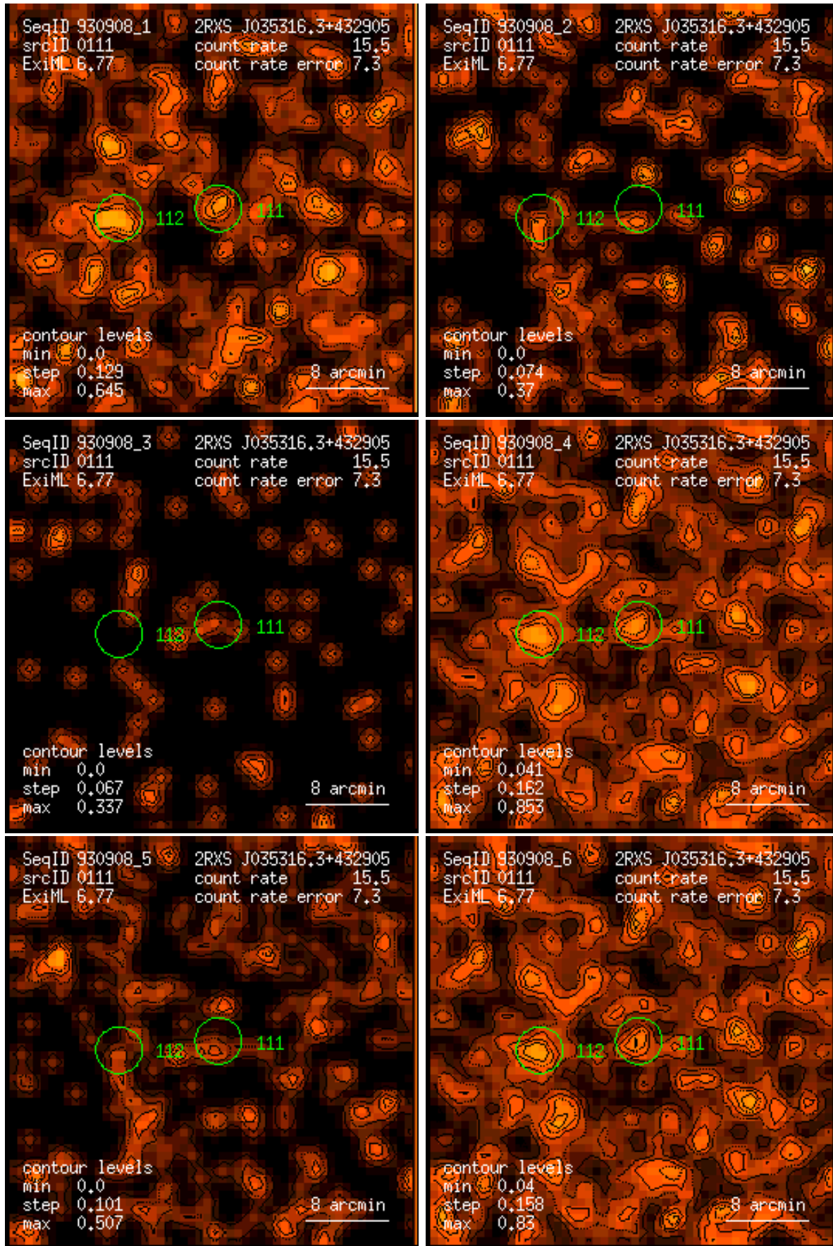
Figure 111: RASS 930908: detection 0111: band rate images, Gaussian filter: (1) PSPC channels 11 – 41, (2) 52 – 90, (3) 91 – 201, (4) 11 – 235, (5) 52 – 201, (6) 11 – 201. Broad band rates in counts/ks. Band rate contour levels in counts/ks/arcmin 2 .
