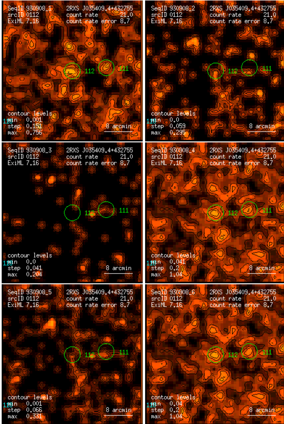
Figure 112: RASS 930908: detection 0112: band rate images, Gaussian filter: (1) PSPC channels 11 – 41, (2) 52 – 90, (3) 91 – 201, (4) 11 – 235, (5) 52 – 201, (6) 11 – 201. Broad band rates in counts/ks. Band rate contour levels in counts/ks/arcmin 2 .
