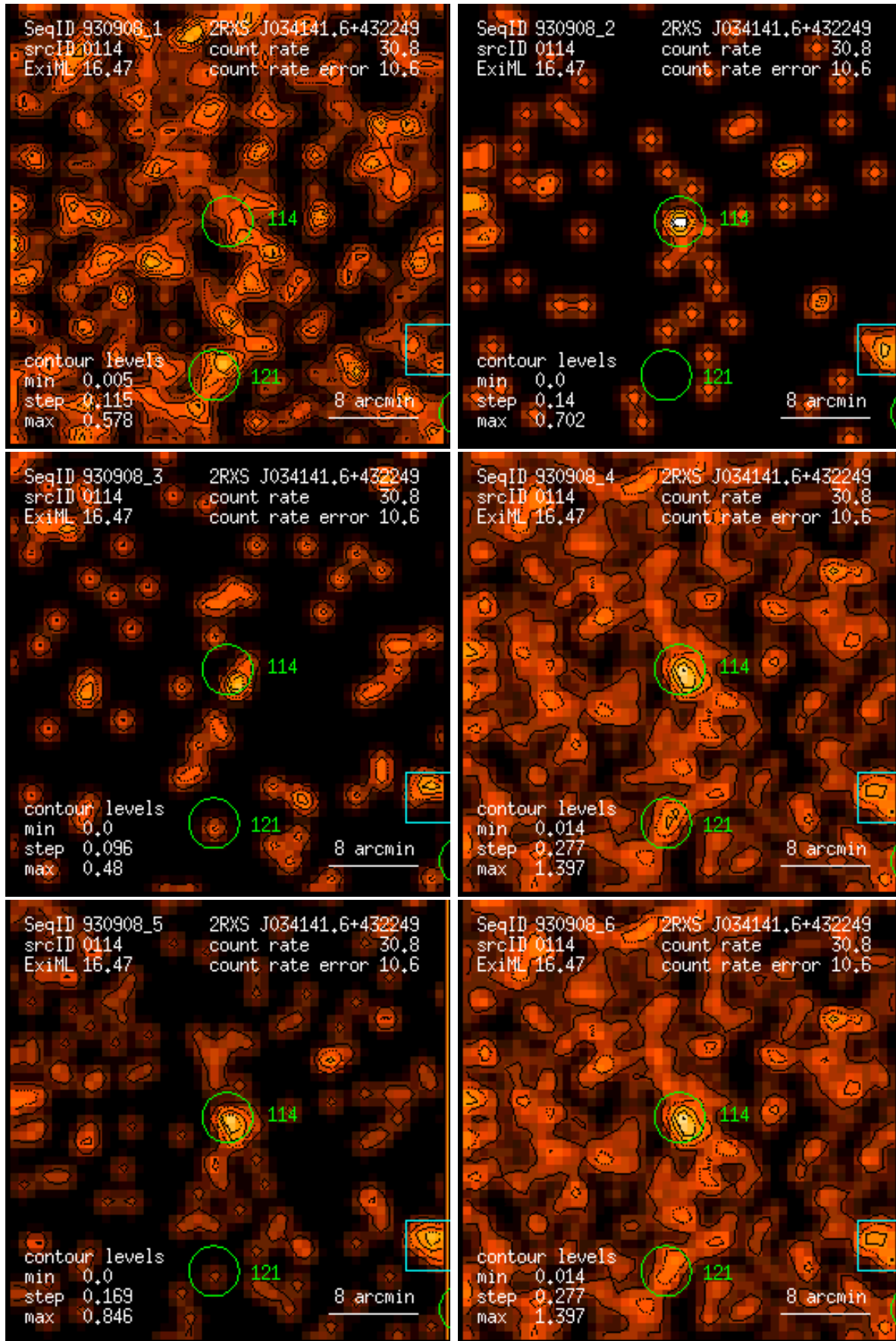
Figure 114: RASS 930908: detection 0114: band rate images, Gaussian filter: (1) PSPC channels 11 – 41, (2) 52 – 90, (3) 91 – 201, (4) 11 – 235, (5) 52 – 201, (6) 11 – 201. Broad band rates in counts/ks. Band rate contour levels in counts/ks/arcmin 2 .
