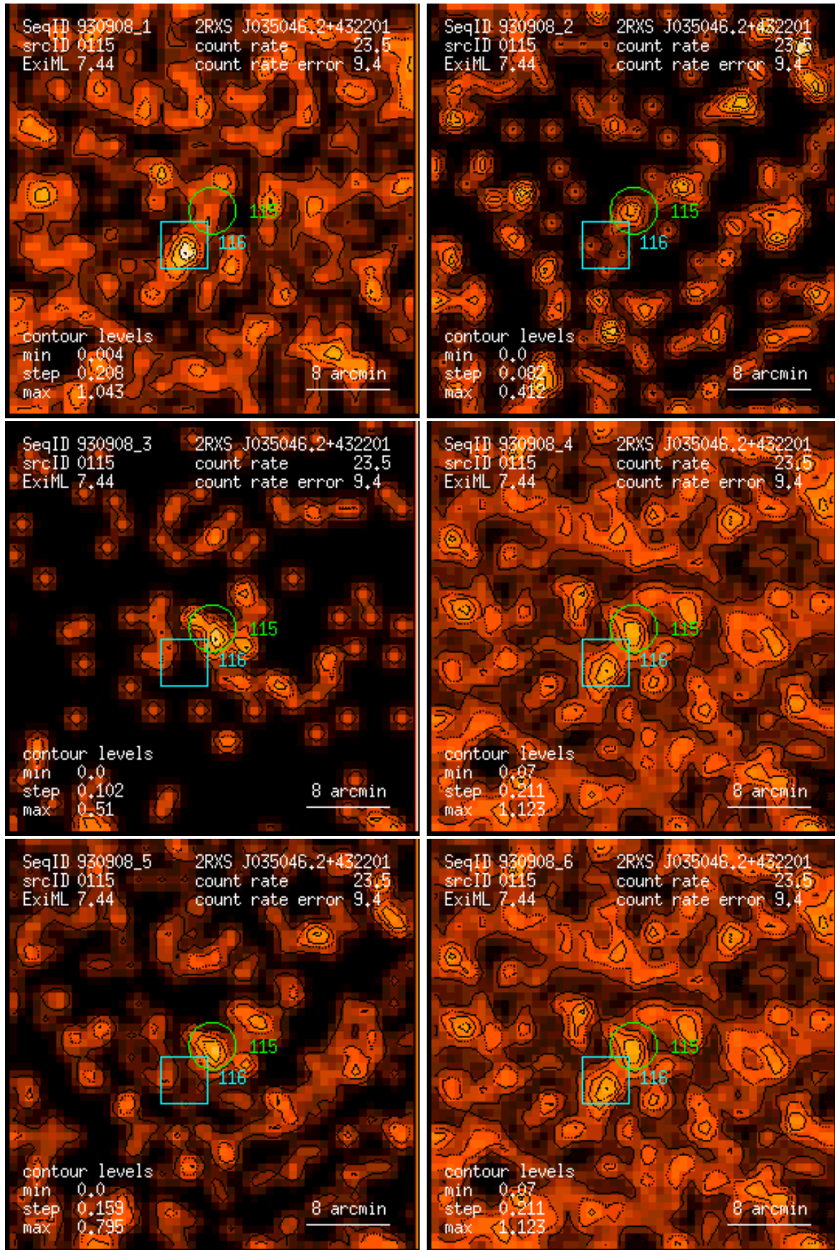
Figure 115: RASS 930908: detection 0115: band rate images, Gaussian filter: (1) PSPC channels 11 – 41, (2) 52 – 90, (3) 91 – 201, (4) 11 – 235, (5) 52 – 201, (6) 11 – 201. Broad band rates in counts/ks. Band rate contour levels in counts/ks/arcmin 2 .
