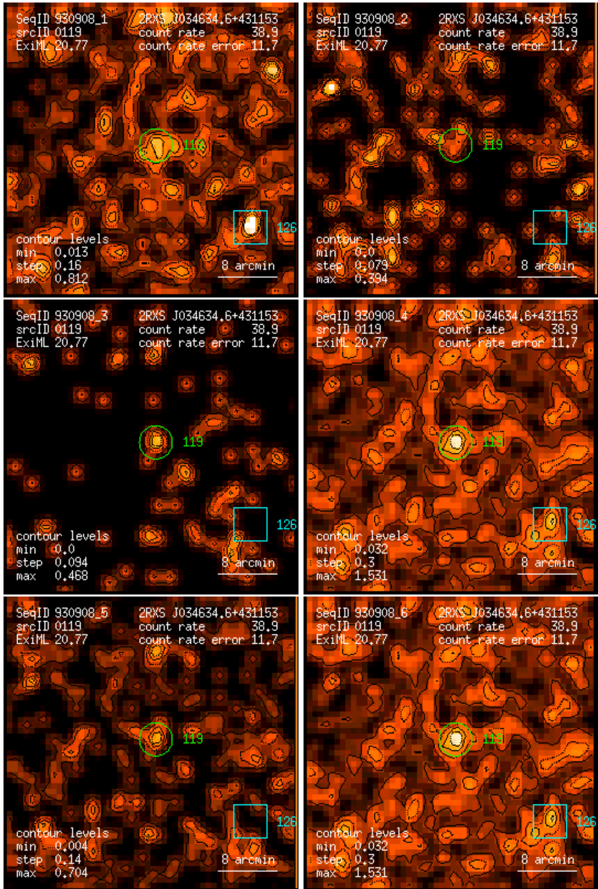
Figure 119: RASS 930908: detection 0119: band rate images, Gaussian filter: (1) PSPC channels 11 – 41, (2) 52 – 90, (3) 91 – 201, (4) 11 – 235, (5) 52 – 201, (6) 11 – 201. Broad band rates in counts/ks. Band rate contour levels in counts/ks/arcmin 2 .
