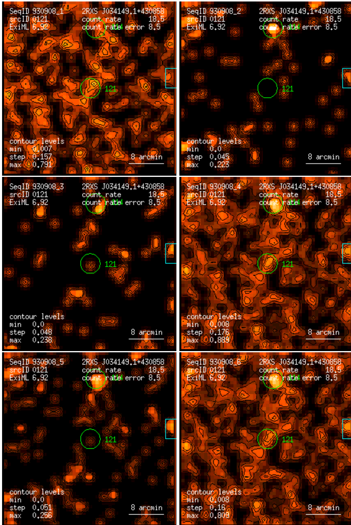
Figure 121: RASS 930908: detection 0121: band rate images, Gaussian filter: (1) PSPC channels 11 – 41, (2) 52 – 90, (3) 91 – 201, (4) 11 – 235, (5) 52 – 201, (6) 11 – 201. Broad band rates in counts/ks. Band rate contour levels in counts/ks/arcmin 2 .
