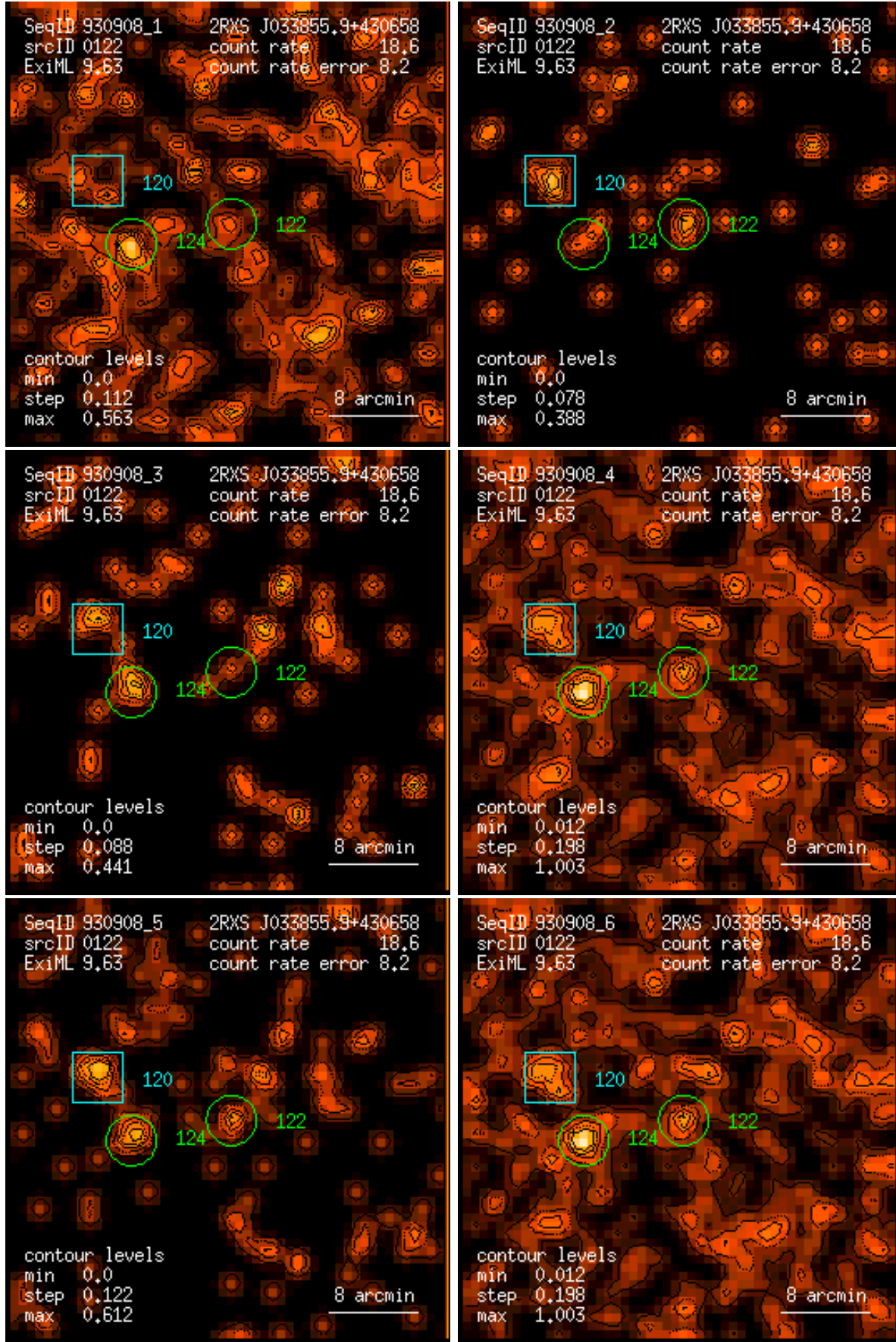
Figure 122: RASS 930908: detection 0122: band rate images, Gaussian filter: (1) PSPC channels 11 – 41, (2) 52 – 90, (3) 91 – 201, (4) 11 – 235, (5) 52 – 201, (6) 11 – 201. Broad band rates in counts/ks. Band rate contour levels in counts/ks/arcmin 2 .
