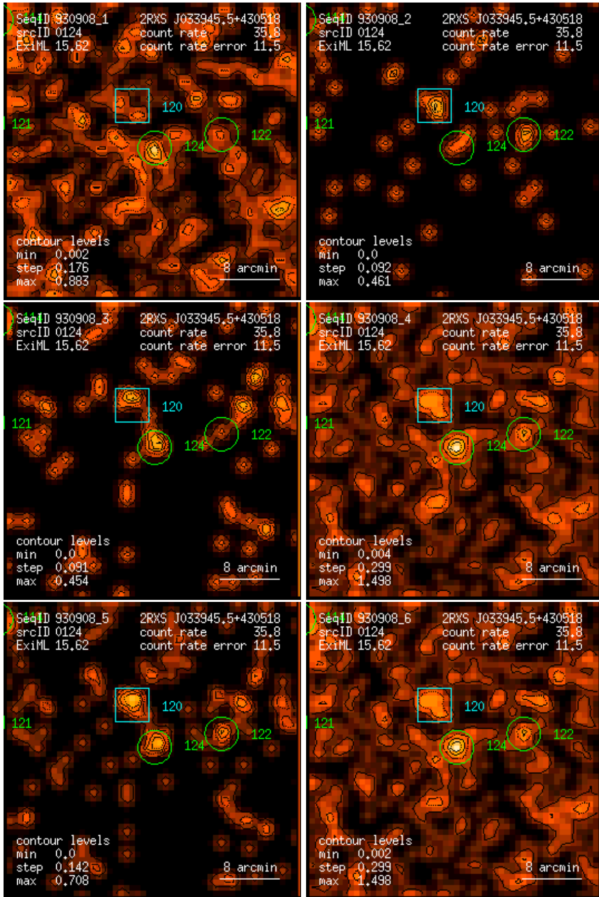
Figure 124: RASS 930908: detection 0124: band rate images, Gaussian filter: (1) PSPC channels 11 – 41, (2) 52 – 90, (3) 91 – 201, (4) 11 – 235, (5) 52 – 201, (6) 11 – 201. Broad band rates in counts/ks. Band rate contour levels in counts/ks/arcmin 2 .
