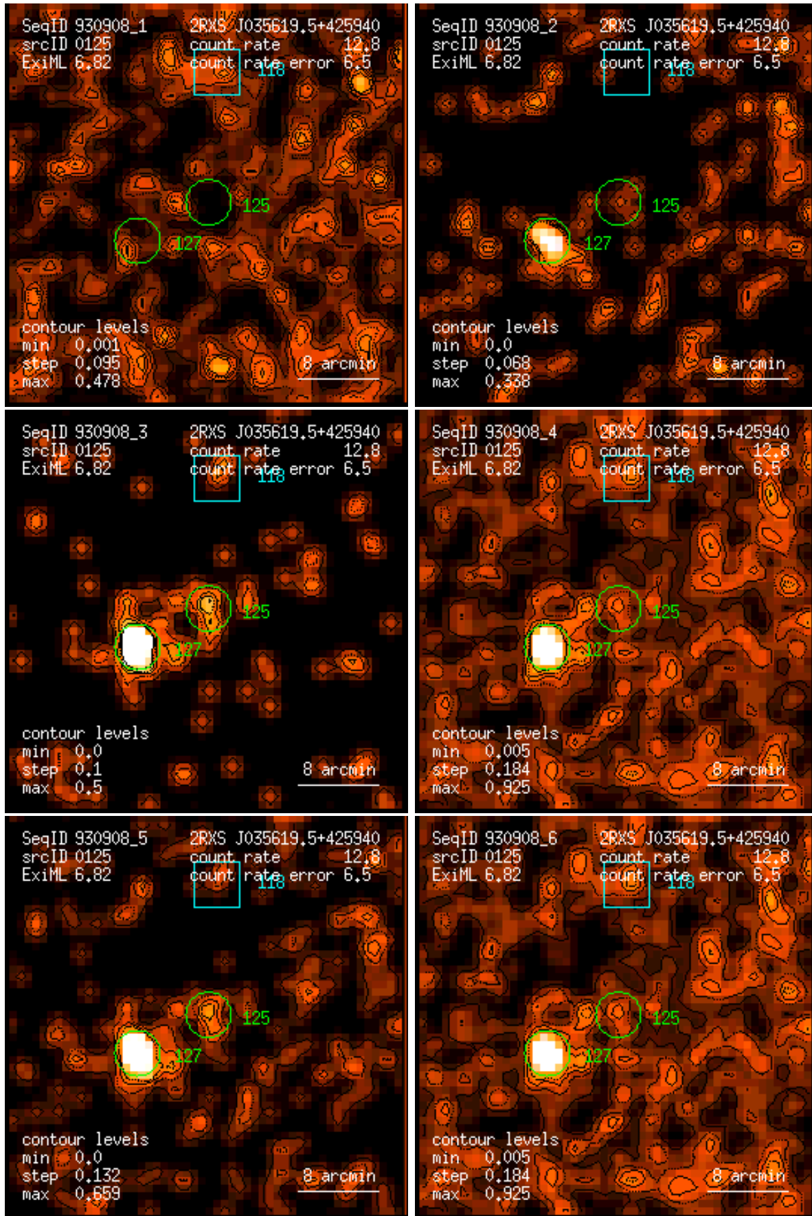
Figure 125: RASS 930908: detection 0125: band rate images, Gaussian filter: (1) PSPC channels 11 – 41, (2) 52 – 90, (3) 91 – 201, (4) 11 – 235, (5) 52 – 201, (6) 11 – 201. Broad band rates in counts/ks. Band rate contour levels in counts/ks/arcmin 2 .
