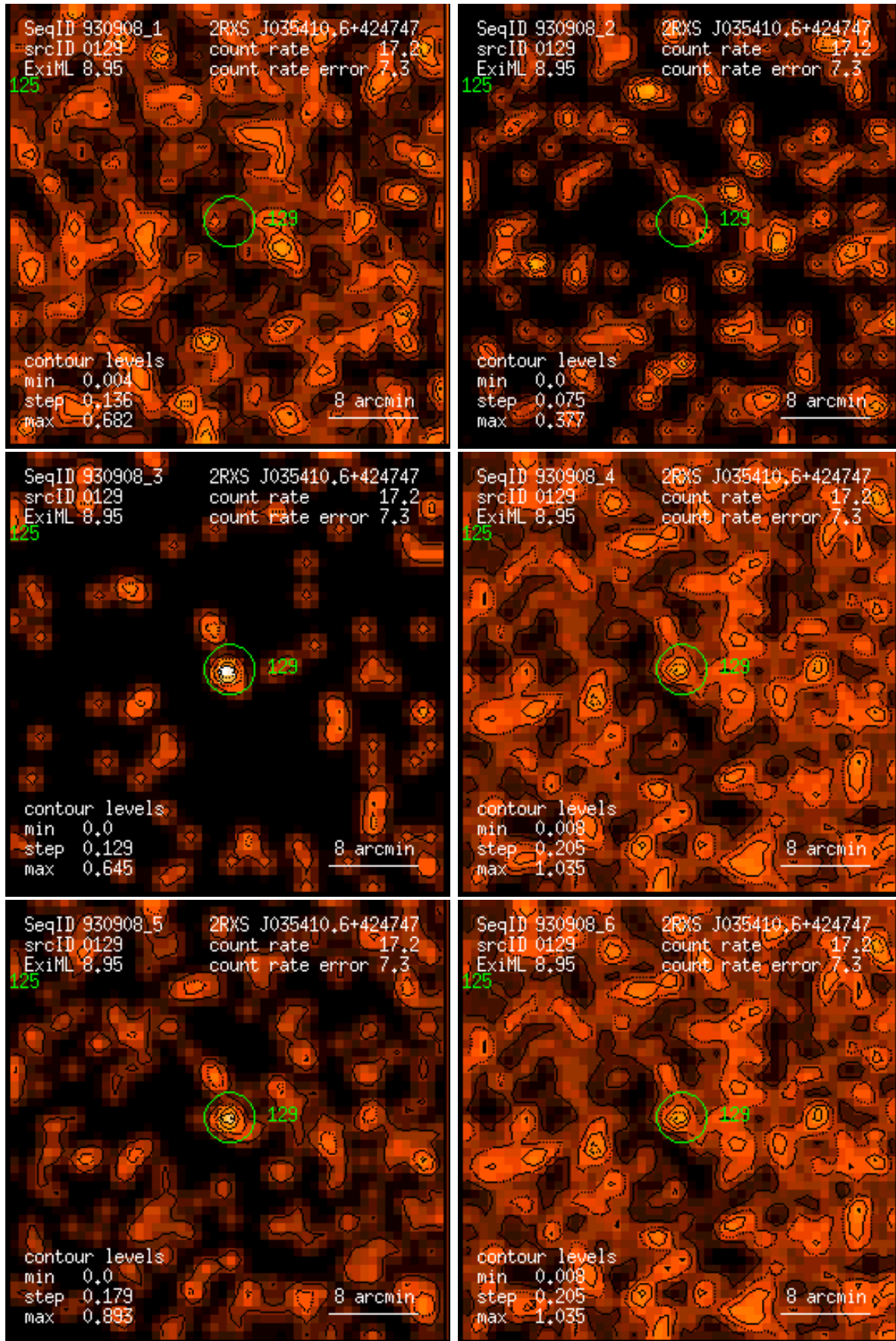
Figure 129: RASS 930908: detection 0129: band rate images, Gaussian filter: (1) PSPC channels 11 – 41, (2) 52 – 90, (3) 91 – 201, (4) 11 – 235, (5) 52 – 201, (6) 11 – 201. Broad band rates in counts/ks. Band rate contour levels in counts/ks/arcmin 2 .
