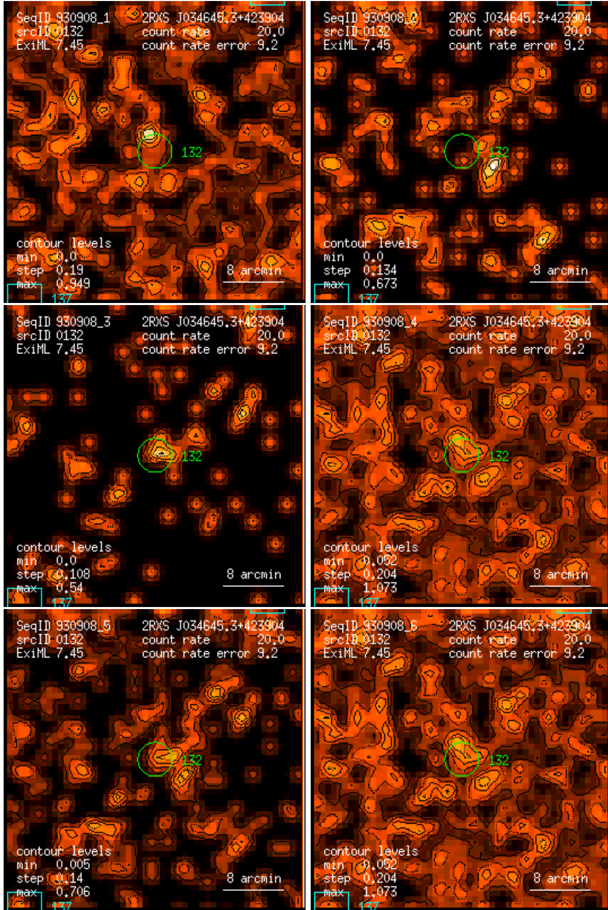
Figure 132: RASS 930908: detection 0132: band rate images, Gaussian filter: (1) PSPC channels 11 – 41, (2) 52 – 90, (3) 91 – 201, (4) 11 – 235, (5) 52 – 201, (6) 11 – 201. Broad band rates in counts/ks. Band rate contour levels in counts/ks/arcmin 2 .
