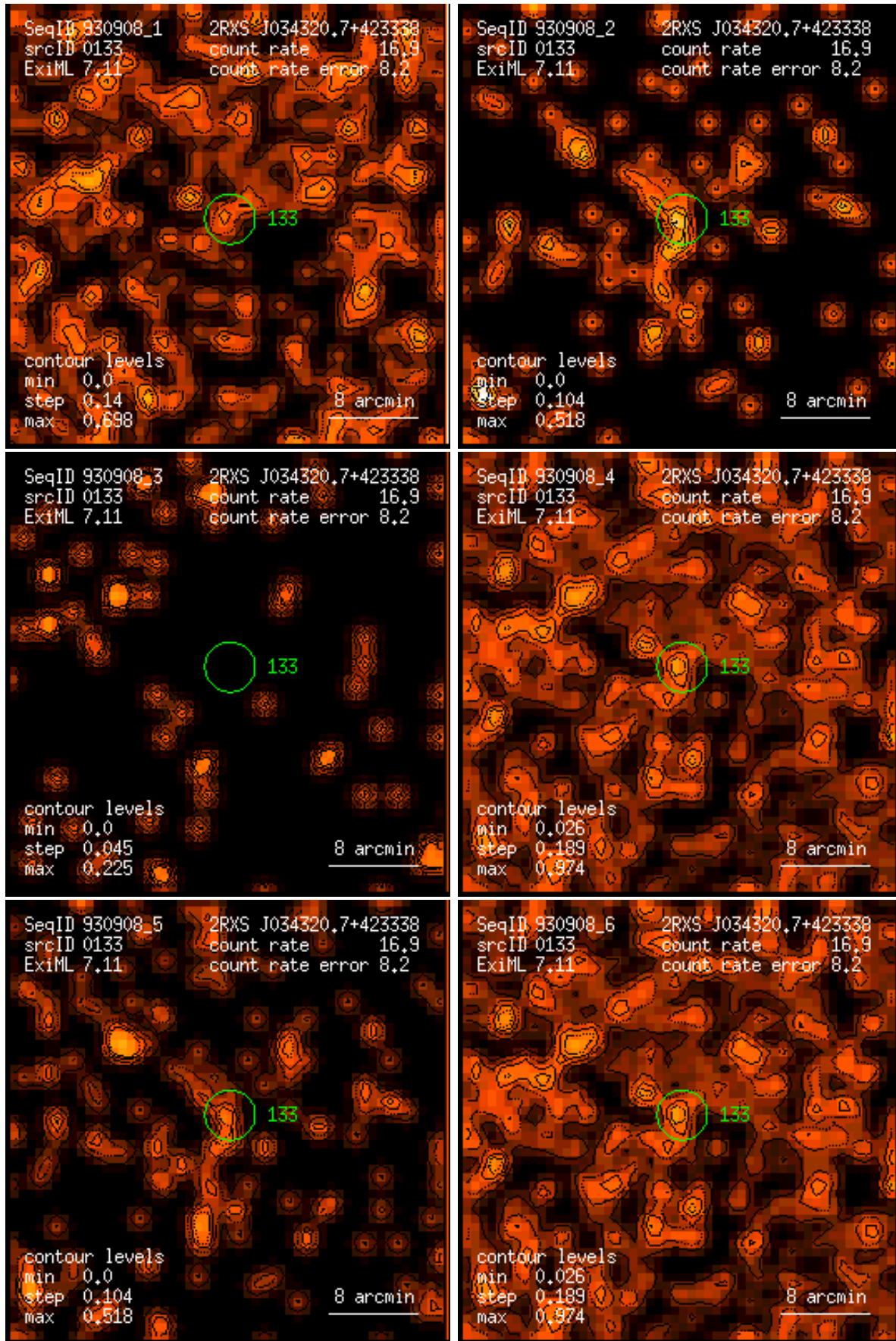
Figure 133: RASS 930908: detection 0133: band rate images, Gaussian filter: (1) PSPC channels 11 – 41, (2) 52 – 90, (3) 91 – 201, (4) 11 – 235, (5) 52 – 201, (6) 11 – 201. Broad band rates in counts/ks. Band rate contour levels in counts/ks/arcmin 2 .
