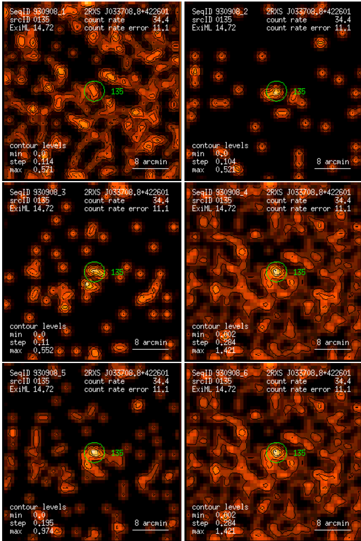
Figure 135: RASS 930908: detection 0135: band rate images, Gaussian filter: (1) PSPC channels 11 – 41, (2) 52 – 90, (3) 91 – 201, (4) 11 – 235, (5) 52 – 201, (6) 11 – 201. Broad band rates in counts/ks. Band rate contour levels in counts/ks/arcmin 2 .
