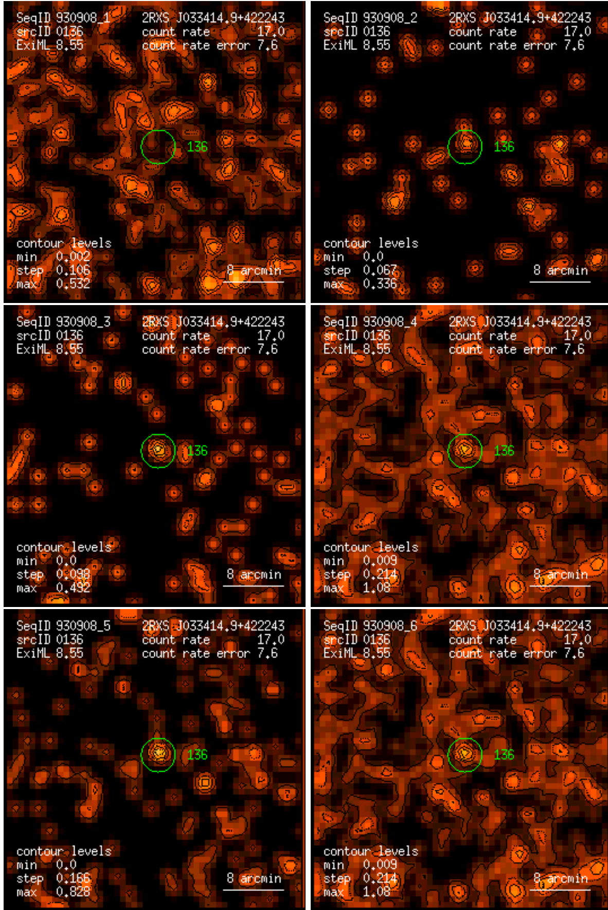
Figure 136: RASS 930908: detection 0136: band rate images, Gaussian filter: (1) PSPC channels 11 – 41, (2) 52 – 90, (3) 91 – 201, (4) 11 – 235, (5) 52 – 201, (6) 11 – 201. Broad band rates in counts/ks. Band rate contour levels in counts/ks/arcmin 2 .
