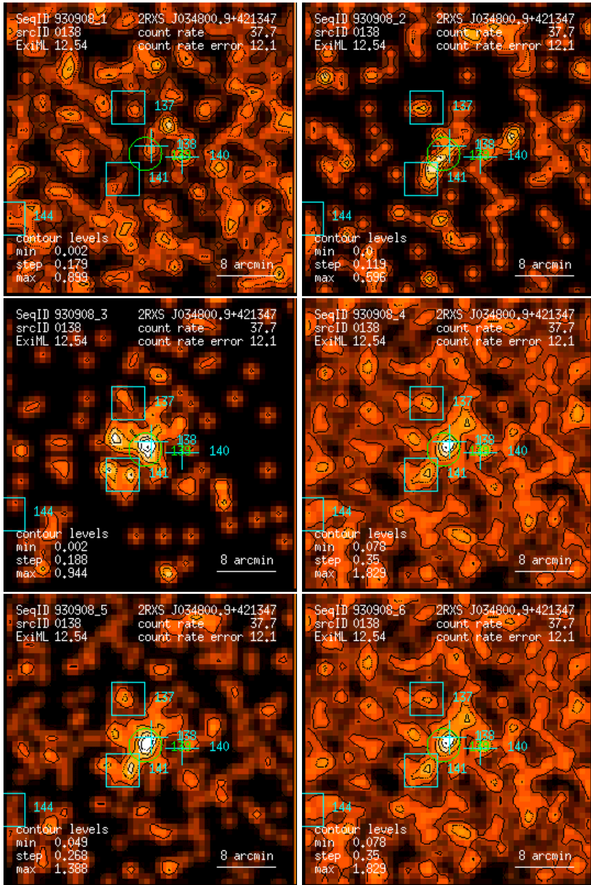
Figure 138: RASS 930908: detection 0138: band rate images, Gaussian filter: (1) PSPC channels 11 – 41, (2) 52 – 90, (3) 91 – 201, (4) 11 – 235, (5) 52 – 201, (6) 11 – 201. Broad band rates in counts/ks. Band rate contour levels in counts/ks/arcmin 2 .
